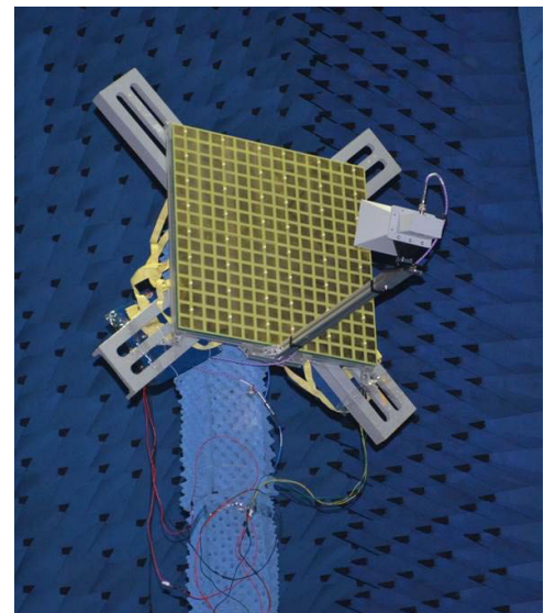
FIGURE 5. Photograph of the fabricated RIS having 16 \times 16 2-bit elements.
