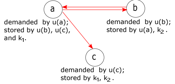
Fig. 3: Directed graph of the two-sender ( k_1 and k_2 ) distributed index problem in Proposition 1. A direct edge from node a to node b , means that receiver u(b) demanding message b stores message a demanded by receiver u(a) .
