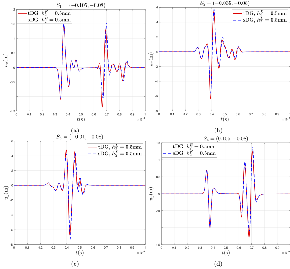
Figure 4: Comparison of displacement components calculated by the tDG solver and the sDG solver on the finer mesh.
