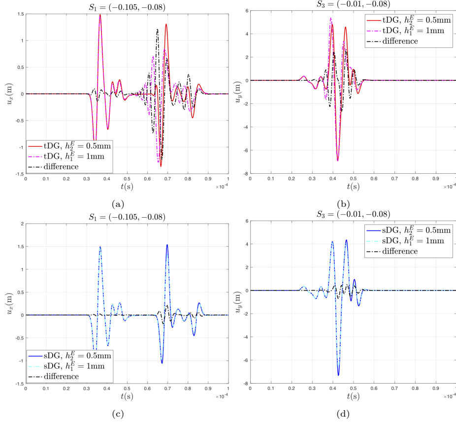
Figure 5: Comparison of displacement components calculated with two different mesh sizes.
