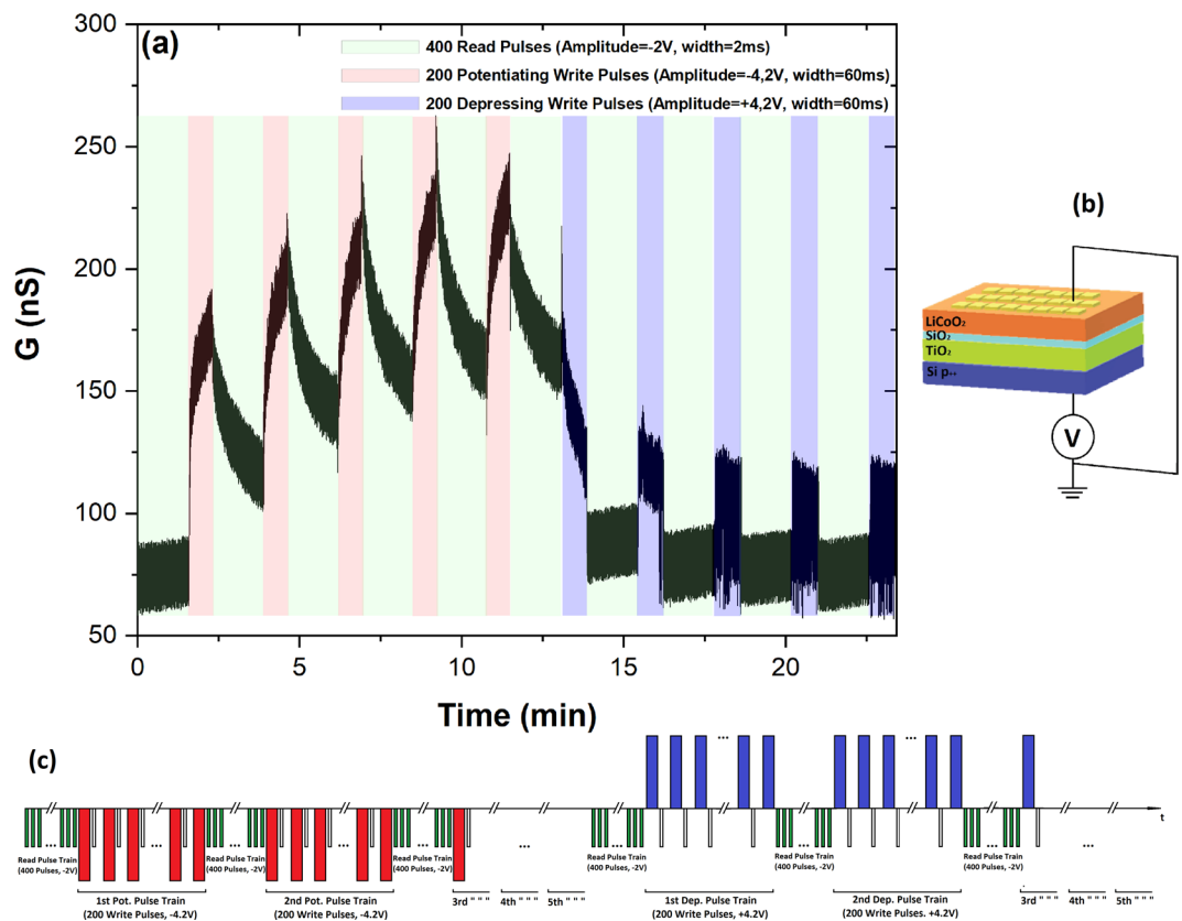
Figure 4. Conductance enhancement, relaxation and depression during voltage pulse stimulation. Pulsed stimulation, of the Au/Li x CoO 2 /SiO x /TiO 2 /p + -Si device with potentiating and depressing voltage pulse trains (write: -/+4.2 V, pulse width: 60 ms) while monitoring the conductance modulation (read: -2 V; pulse width: 2 ms), (top Au electrode: 300 × 300 μm 2 ). Stimulated enhancement and subsequent conductance relaxation along with stimulated conductance depression can be observed (a). Schematics of the measurement setup (b) and the read/write pulse sequence applied on the device (c) are also illustrated.
