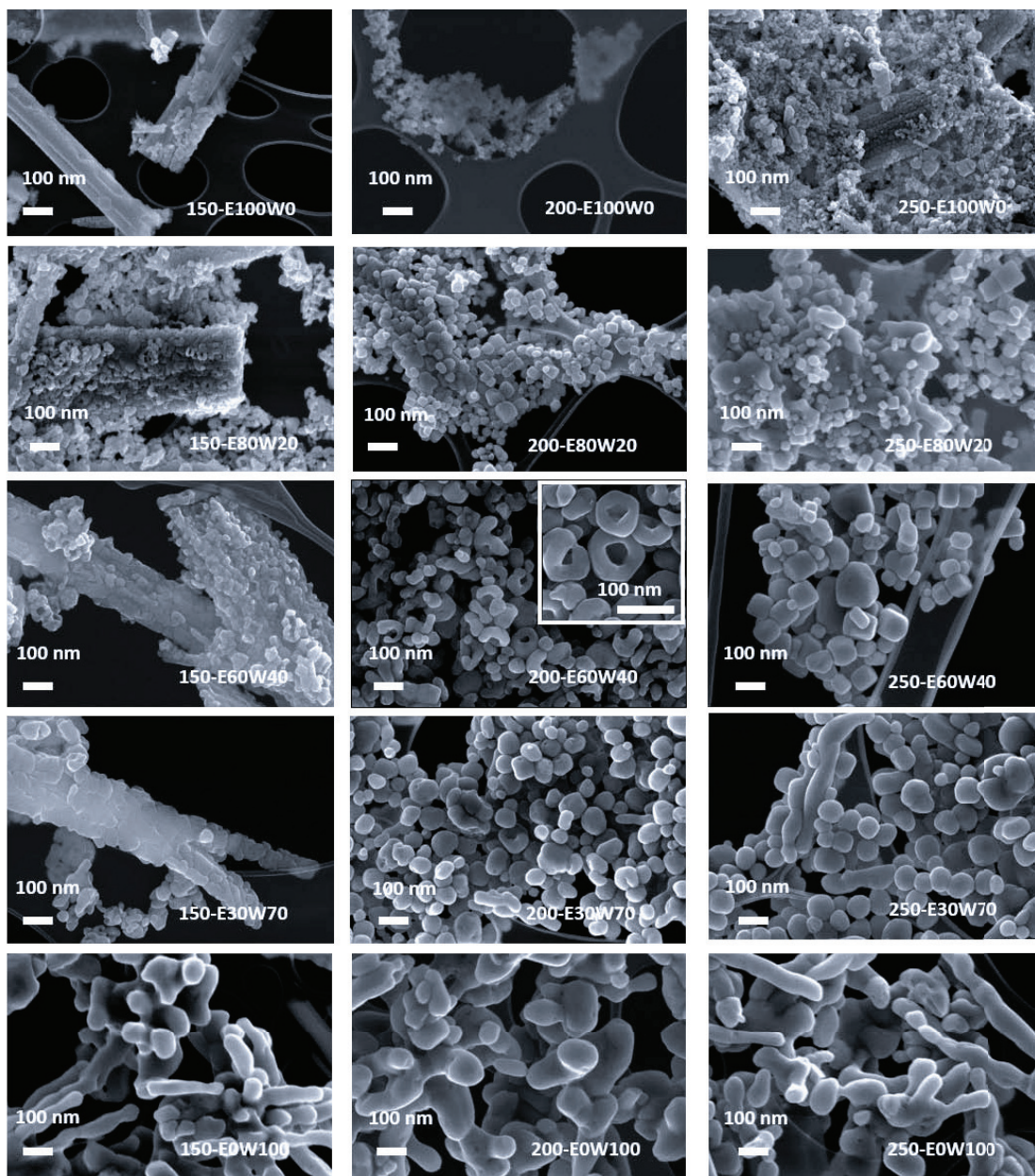
Figure 3: SEM images of the as-prepared BaTiO 3 products obtained after 24 hours at 150°C (left column), 200°C (middle column) and 250°C (right column) for the various solvent compositions (ExW100 - x).
