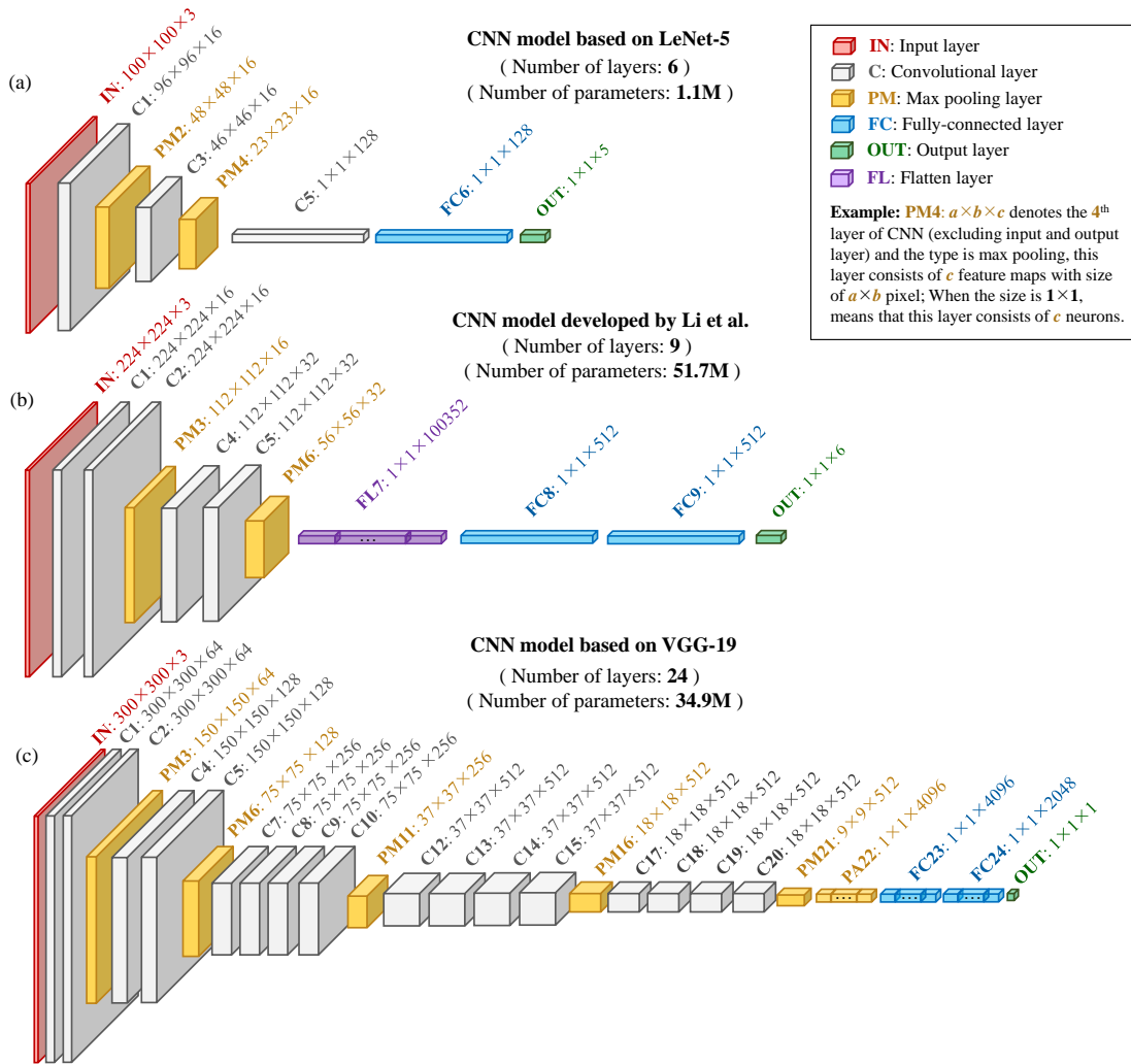
Fig. 2 Examples of CNN structures adopted for PV FDD: (a) LeNet-5 [77] (low number of layers and low number of parameters), (b) Li et al. scheme [71] (low number of layers and high number of parameters), (c) VGG-19 [72] (high number of layers and high number of parameters).
