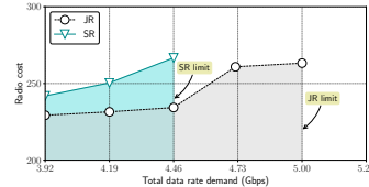
Fig. 12. Maximum supported data rate associated to the SR and JR provisioning approaches when 3 slices of type 1, 2, and 3 have to be deployed.
