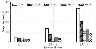
Fig. 10. Computing time of the 4 proposed provisioning variants
