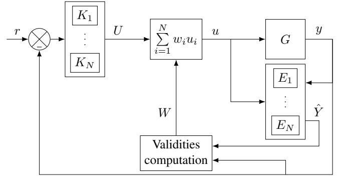
Fig. 1. MMAC method
