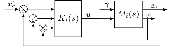
Fig. 4. Three degree of freedom control loop
