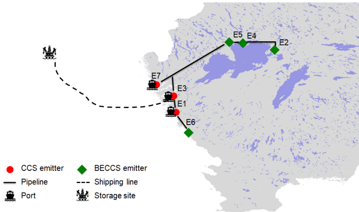
Figure 3: The least costly infrastructure connecting the seven industrial emitters
