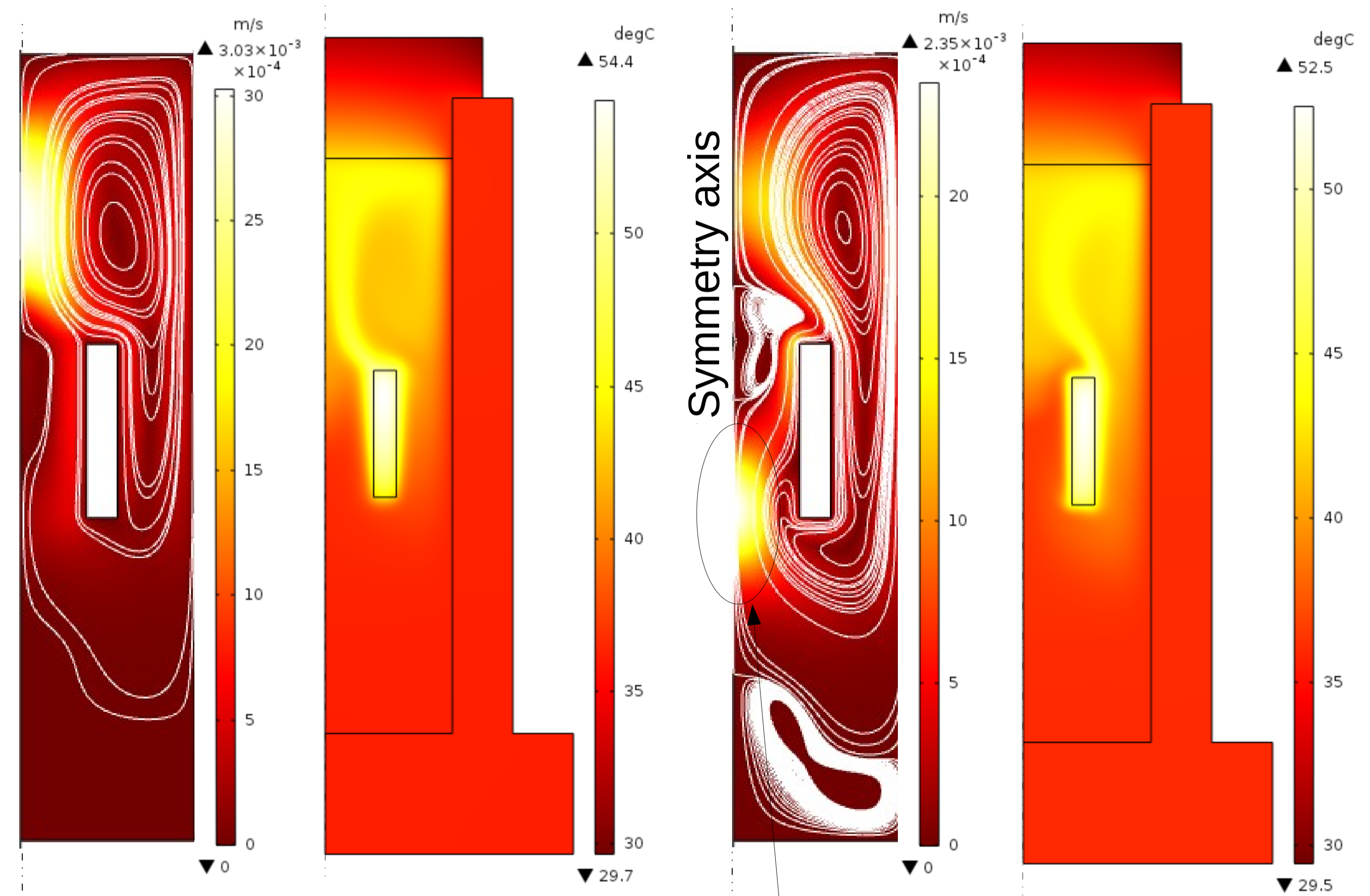
Without Helmholtz force With Helmholtz force New convection cell
