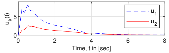
(c) Control input u
