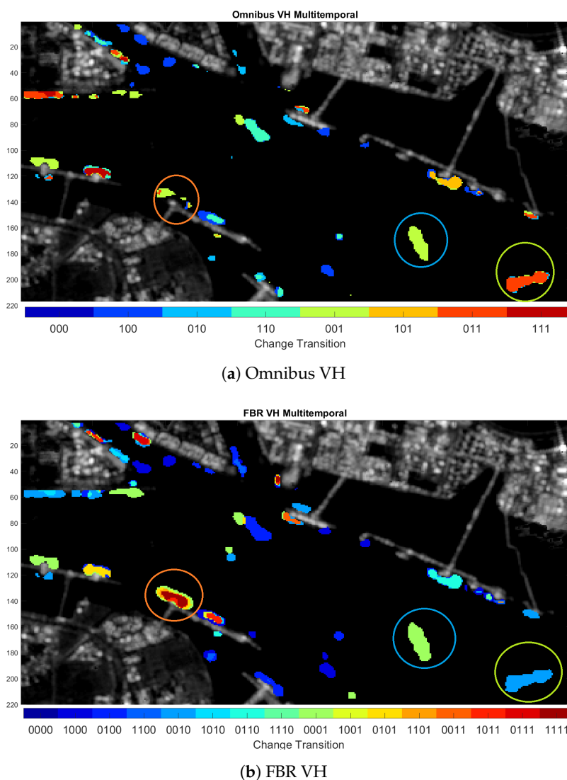
Figure 19. (a) Four dates Omnibus change detection analysis, (b) CD FBR computation on the four first dates.
