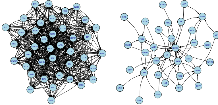
Figure 3: Examples of prediction network inferred with knockoffs. T_{in} = 300 trading days, period ending on 2006-03-13. Left plot: FDR= 0.3 and 100 runs per asset; right plot: FDR= 0.2 and 10 runs per asset. Selection via random forest variable importance.
