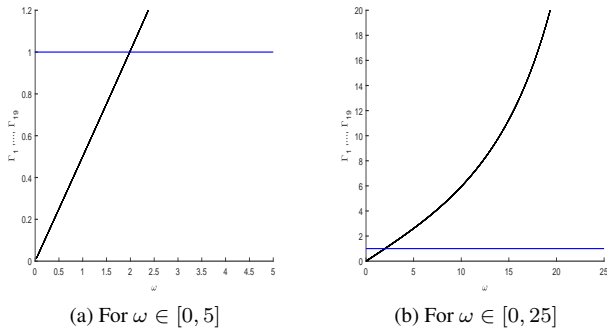
FIGURE 7. FSCs when d_1 = d_2 = 0.1 for Example 2
