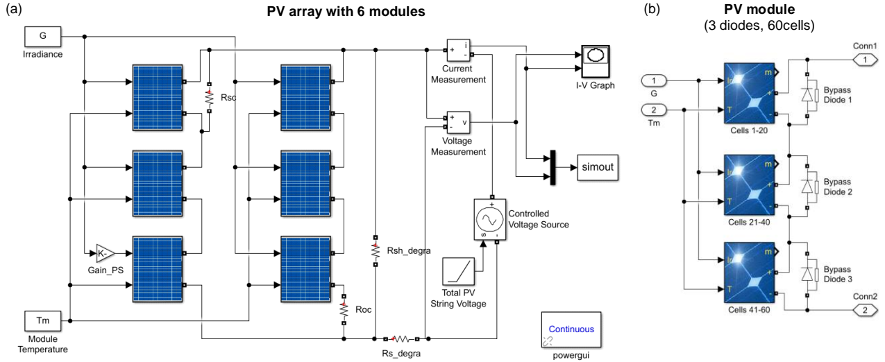
Fig. 1 Simulation model: (a) PV array structure, (b) PV module structure
