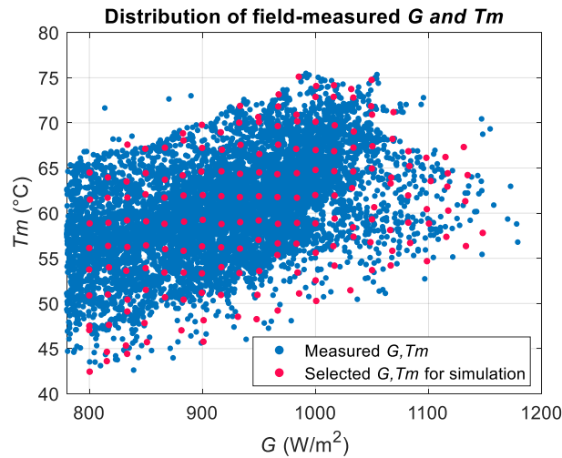
169 170 Fig. 2 Selected G and T_m based on field-measurement during summer for one mc-Si PV module
