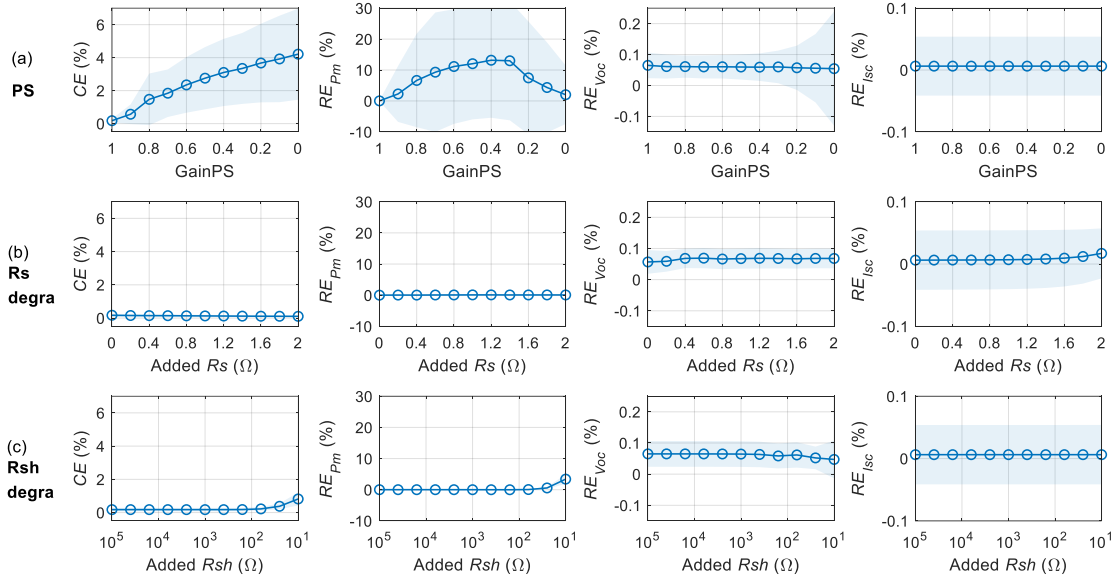
Fig. 12 CE and RE of P_m , V_{oc} and I_{sc} for M3 under 3 faulty cases with variable fault severity: (a) PS, (b) R_s degradation, (c) R_{sh} degradation (the circled line represents the mean value for the 120 corrected curves for each fault severity, while the band area behind represents the standard deviation; the x -axis for R_{sh} degradation is set as log scale; the degree of severity is presented from healthy to severe on the x -axis from left to right)
