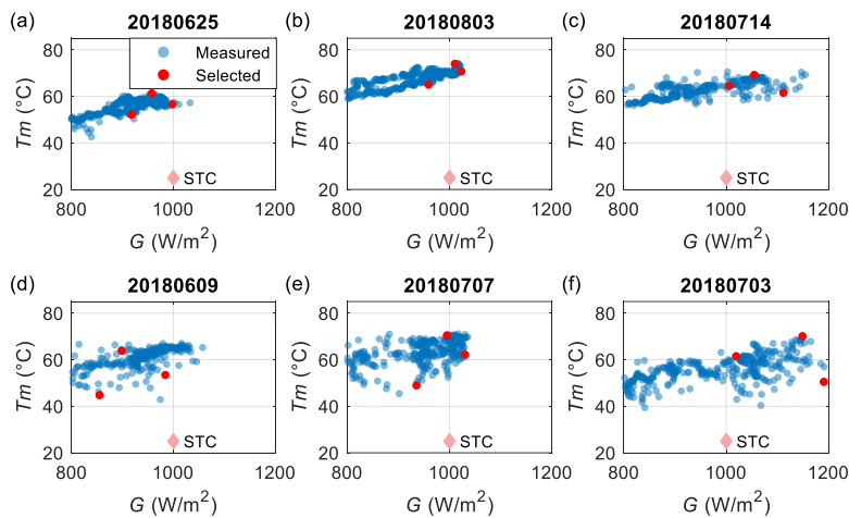
341 Fig. 9 Examples of selected G and T_m from different summer days: (a, b, c) clear sunny days, (d, e, f) cloudy days ((a, d): the 3 342 selected G < 1000 W/m 2 , (b, e): selected G around 1000 W/m 2 , (c, f): selected G > 1000 W/m 2 )
