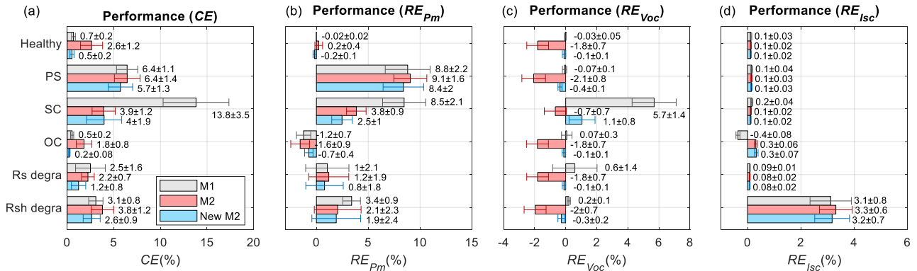
239 Fig. 4 Four metrics to present the correction performance of M1, M2 and NewM2: (a) CE , (b) RE of P_m , (c) RE of V_{oc} , (d) RE of 240 I_{SC} (the bars represent the mean value for the correction of 174 curves, while the horizontal whiskers represent the standard deviation 241 (std), these 2 values are marked as 'mean' ± 'std') 242
