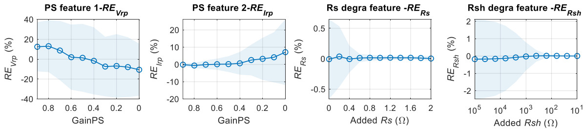
397 Fig. 15 RE of fault features under PS, R_s and R_{sh} degradations for fault of variable severity using M3 (the circled line represents the 398 mean, while the band area represents the standard deviation) 399
