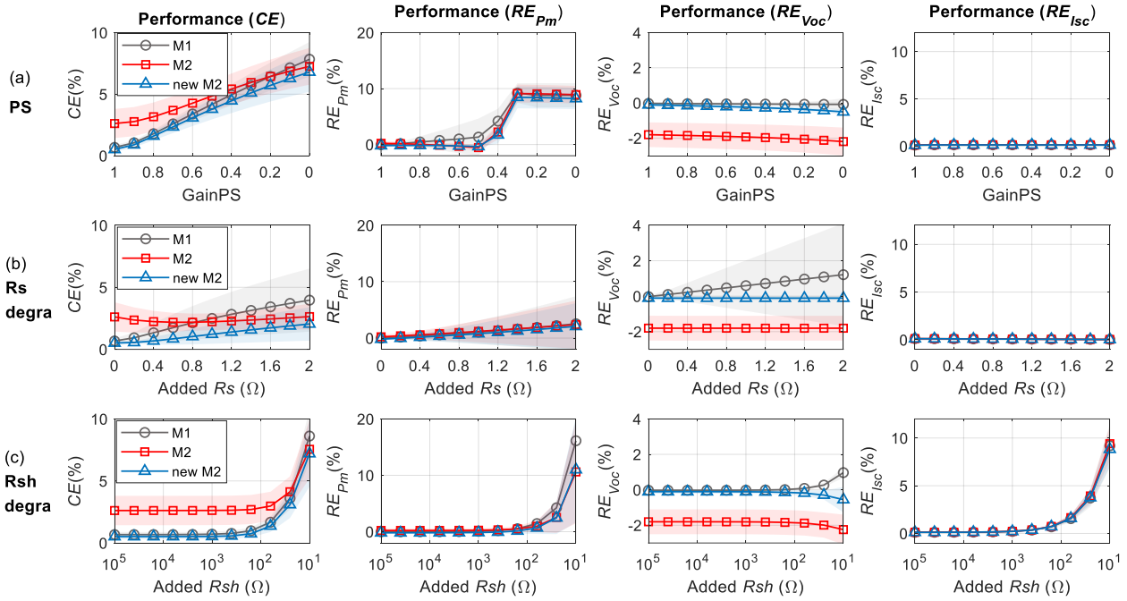
286 287 Fig. 5 CE and RE of P_m , V_{oc} and I_{sc} using M1, M2 and NewM2 under 3 faulty conditions with variable fault severity: (a) PS, (b) Rs 288 degradation, (c) Rsh degradation (the marked line represents the mean of 174 values obtained from the correction of 174 under each 289 fault severity, while the band area behind represents the standard deviation; the x -axis for Rsh degradation is set as log scale; the 290 degree of severity is presented from healthy to severe on the x -axis from left to right)
