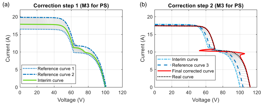
Fig. 11 Correction procedure under PS using 3 reference curves-based M3: (a) correction step 1, (b) correction step 2
