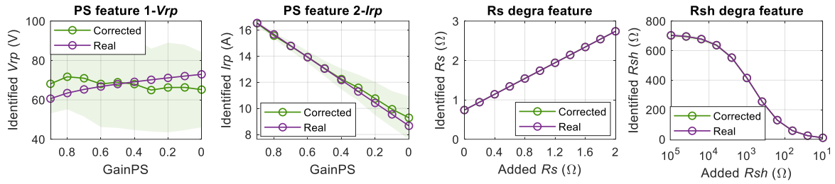
391 Fig. 14 Identified feature from corrected (using M3) and original I-V curve for fault of variable severity (the circled line represents the 392 mean, while the band area represents the standard deviation; the values of R_s or R_{sh} identified from I-V curve are not equal to the 393 additional resistance (illustrated in Fig. 1) due to the existence of inherent equivalent R_s (0.74 \Omega ) or R_{sh} (708.36 \Omega ) of PV arrays 394
