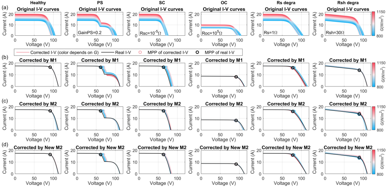
183 184 Fig. 3 Correction results, (a): curves simulated for correction (each condition contains 174 curves with field-measured combinations of 185 G and T_m at constant fault severity), (b): corrected curves using M1, (c): corrected curves using M2, (d): corrected curves using 186 NewM2 (the displayed color of each curve is determined by the irradiance value with the colorbar on the right side of the figure, the 187 circles on the curves represent the MPP)
