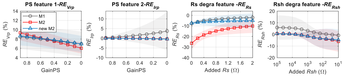
Fig. 7 RE of fault features under PS, R_s and R_{sh} degradations with variable fault severity (the marked line represents the mean of 174 values obtained from the correction of 174 curves under each fault severity, while the band area behind represents the standard deviation; the x -axis for R_{sh} degradation is set as log scale; the degree of severity is presented from healthy (except for V_{rp} and I_{rp} as these features do not exist under healthy condition) to severe on the x -axis from left to right)
