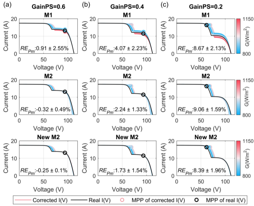
Fig. 6 Corrected curves and RE_{P_m} using M1, M2 and NewM2 under three fault severities of PS: (a) GainPS = 0.6, (b) GainPS = 0.4, (c) GainPS = 0.2 (the displayed color of corrected curves and MPP depends on the G of the curve to correct, the circles on the curves represent the MPP, RE_{P_m} are marked as 'mean'±'std')
