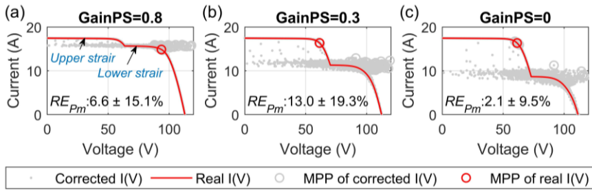
Fig. 13 Corrected curves using M3 under 3 fault severities of PS: (a) GainPS=0.8 , where MPP of real and corrected curves are all at 'lower stair', (b) GainPS = 0.3 , where MPP of real is at 'upper stair' while MPP of most corrected curves at 'lower stair' (c) GainPS = 0 , MPP of real and most corrected curves are all at 'upper stair' (for each case, RE_{P_m} is marked as 'mean'±'std')
