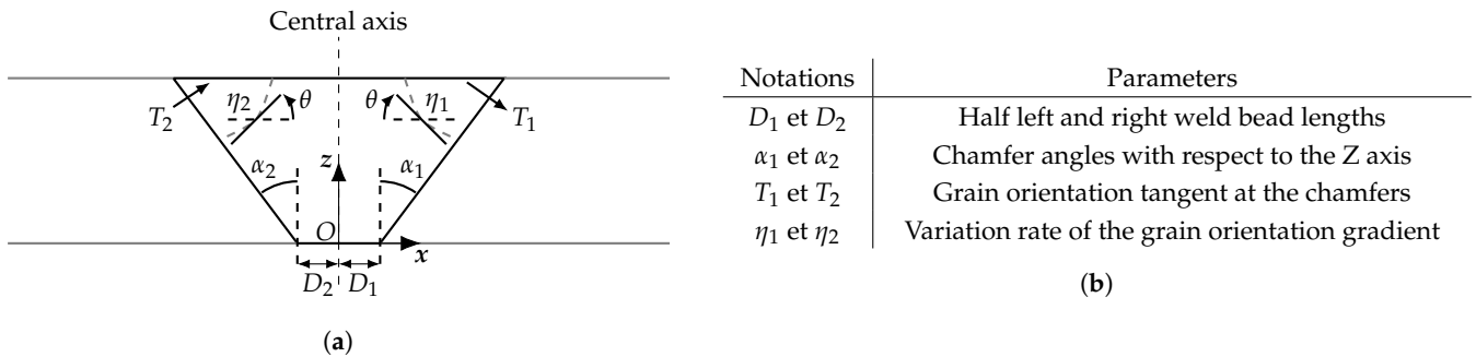
Figure 1. Ogilvy’s model: (a) geometrical description of the model and (b) specific parameters. T_2, D_1 and \alpha_1 are positive values while T_1, D_2 and \alpha_2 are negative values. \eta_1 et \eta_2 always are positive.
