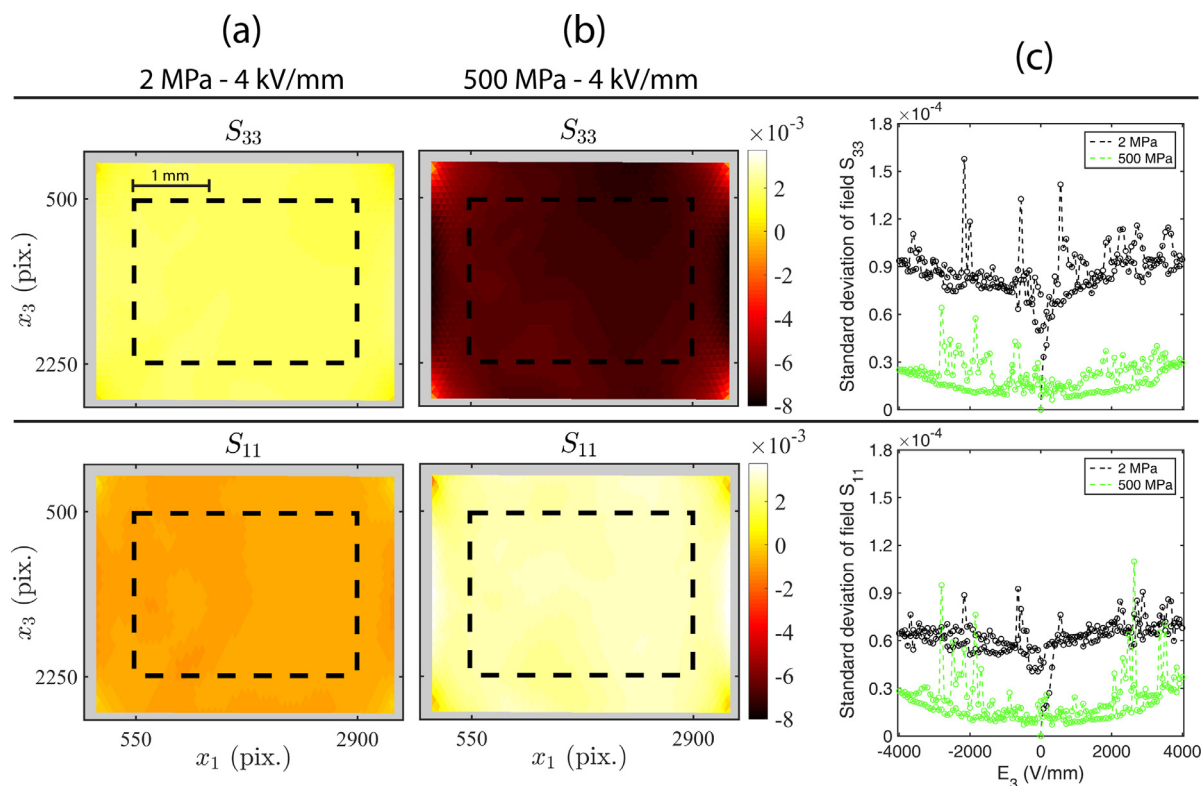
Fig. 2. Longitudinal ( S_{33} ) and transverse ( S_{11} ) DIC strain fields at (2 MPa, 4 kV/mm) (a) and at (500 MPa, 4 kV/mm) (b). Standard deviations of the strain fields S_{33} and S_{11} as a function of the electric field for 2 MPa (black curve) and 500 MPa (green curve) (c). The reference state for fields in (a) and (b) is the material state at 0 V/mm and 2 MPa. (For interpretation of the references to color in this figure legend, the reader is referred to the web version of this article.)
