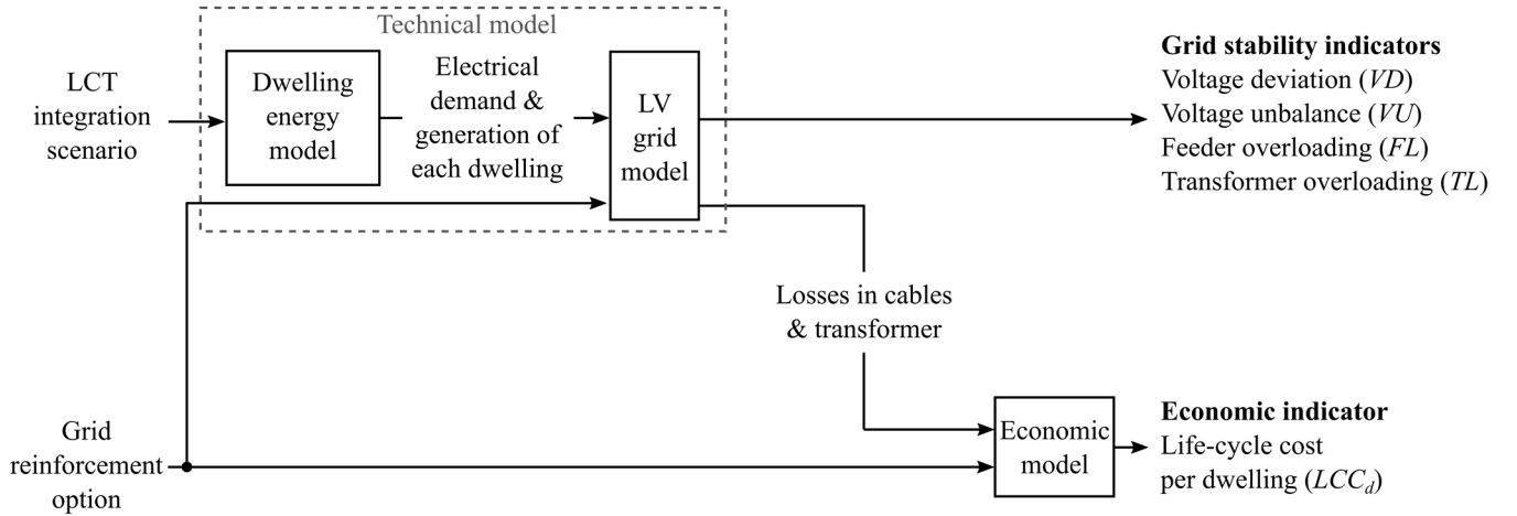
Figure 2 – Evaluation of LCT integration scenarios and grid reinforcement options.
