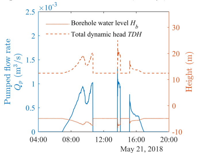
Fig. 7. Simulated pumped flow rate, water level in the borehole and total dynamic head.
