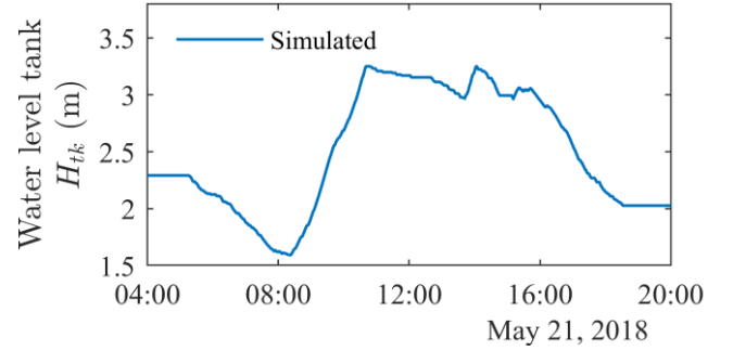
Fig. 9 – Water level in the tank – Simulated – Model output.
