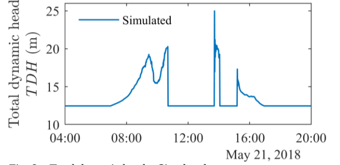
Fig. 8 – Total dynamic head – Simulated.
