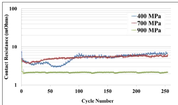
Fig.4 : Contact resistance evolution vs. durability cycles between Au/Ni hemispheres & GCSb flats
