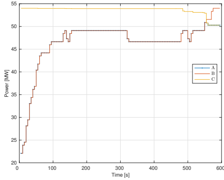
Fig. 4. The power variables in the power generator at node 2745 from the MPC result with prediction horizon N=3 . A) P_n^G(k) ; B) P_n^A(k) ; C) \bar{P}_n^G - P_n^C(k) .
