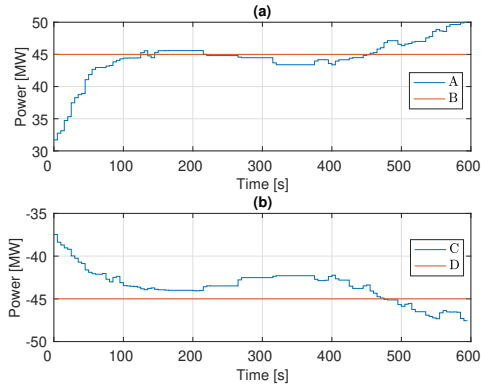
Fig. 3. The power flow on the branches in the open-loop simulation: A) between buses 2745 and 1445; C) between buses 2135 and 2076; B) The maximum power value 45; D) The minimum power value -45.
