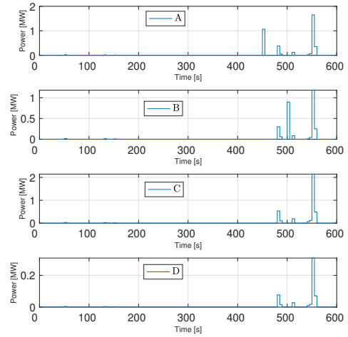
Fig. 6. \Delta P_n^C at the generators. The prediction horizon is N=3 . A) node 10000; B) node 2076; C) node 2745; D) node 4720.
