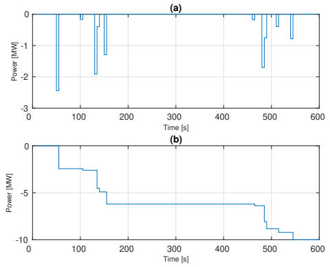
Fig. 5. (a): \Delta P_n^B . (b): P_n^B . The prediction horizon is N=3 .
