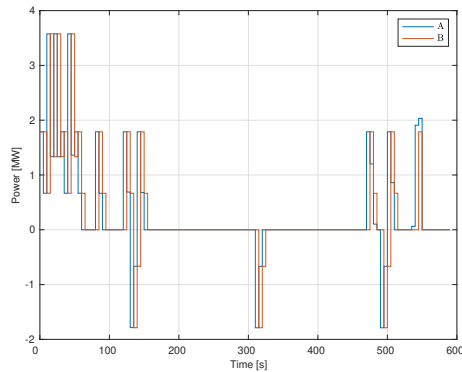
Fig. 7. A) real \Delta P_n^G at the node 2745; B) estimated \Delta P_n^G at the node 2745.
