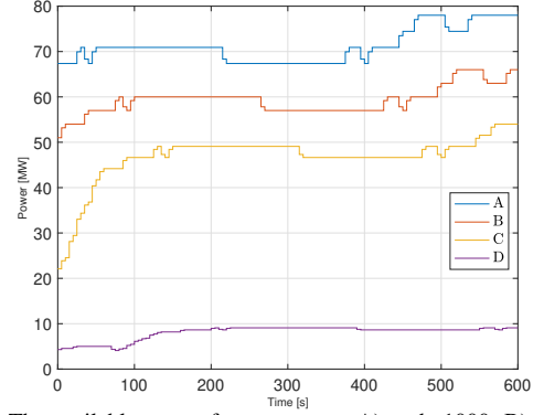
Fig. 2. The available power for generators. A) node 1000; B) node 2076; C) node 2745; D) node 4720.
