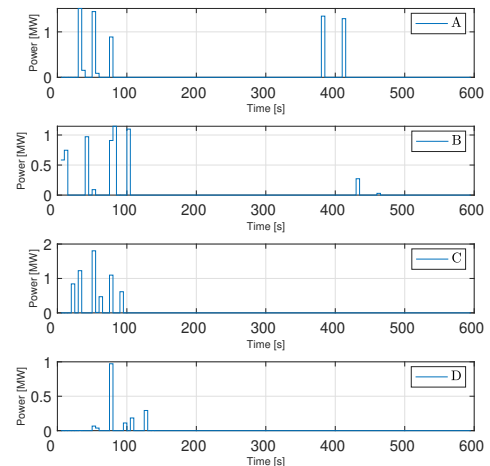
Fig. 9. Control actions for curtailment when prediction horizon N=10 . A) node 10000; B) node 2076; C) node 2745; D) node 4720.
