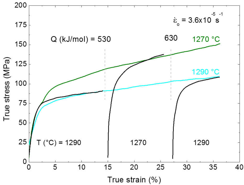
Fig. 11. True stress \sigma - true strain \epsilon curve for BZY deformed at an initial strain rate of 3.6 \times 10^{-5} \text{ s}^{-1} showing two determinations of Q by temperature changes between 1270 and 1290 °C (in black). The corresponding isothermal curves are also displayed (in green and light blue, respectively), which overlap well with the differential curve.
