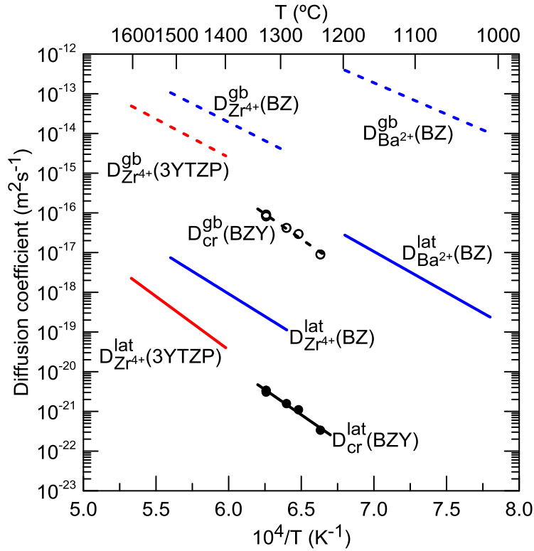
Fig. 14. Effective diffusion coefficients D_{cr}^{lat} and D_{cr}^{gb} for fine-grained 15 at% yttrium-doped barium zirconate (BZY) deduced from deformation data by using Eqs. 2a and 2b (in black). Cation tracer diffusion coefficients of Zr^{4+} and Ba^{2+} in undoped BaZrO_3 (BZ) [39] are also included (in blue). Tracer diffusion coefficients of Zr^{4+} (the creep rate-limiting species) in 3YTZP [34] (in red) are also shown for comparison. (lat = lattice diffusion, gb = grain boundary diffusion).
