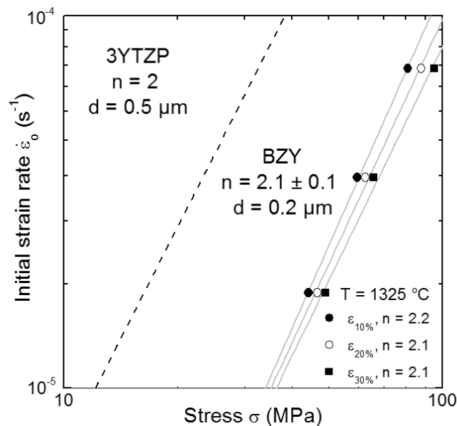
Fig. 9. Variation of strain rate vs stress for BZY at strain levels \epsilon of 10, 20 and 30%. Data for fine-grained ( d = 0.5 \text{ }\mu\text{m} ) 3YTZP with n = 2 , the reference material for superplastic ceramics, is also shown (dashed line) [28].
