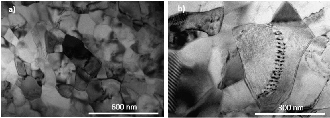
Fig. 8. TEM images of BZY deformed up to 40% at an initial strain rate of 3.6 \times 10^{-5} \text{ s}^{-1} and 1325 °C showing (a) the grain structure and (b) a dislocation pile-up inside a grain.
