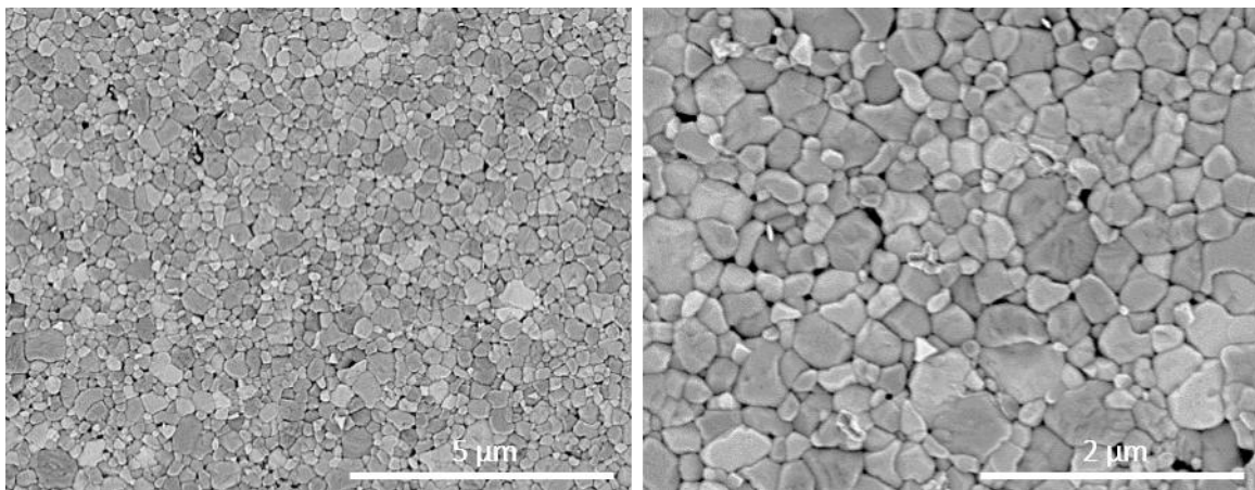
Fig. 2. SEM micrographs of sintered BZY.
