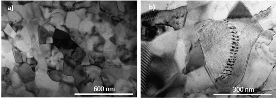
Fig. 8. TEM images of BZY deformed up to 40% at an initial strain rate of 3.6 \times 10^{-5} \text{ s}^{-1} and 1325 \text{ }^\circ\text{C} showing (a) the grain structure and (b) a dislocation pile-up inside a grain.
