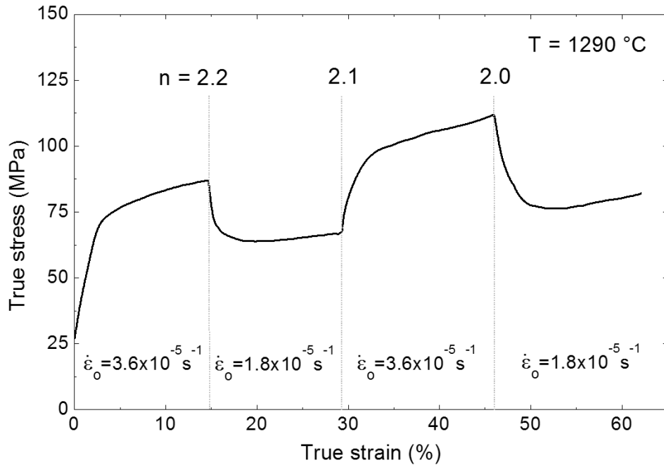
Fig. 10. True stress \sigma - true strain \epsilon curve for BZY deformed at 1290 °C showing several determinations of n by strain rate changes.
