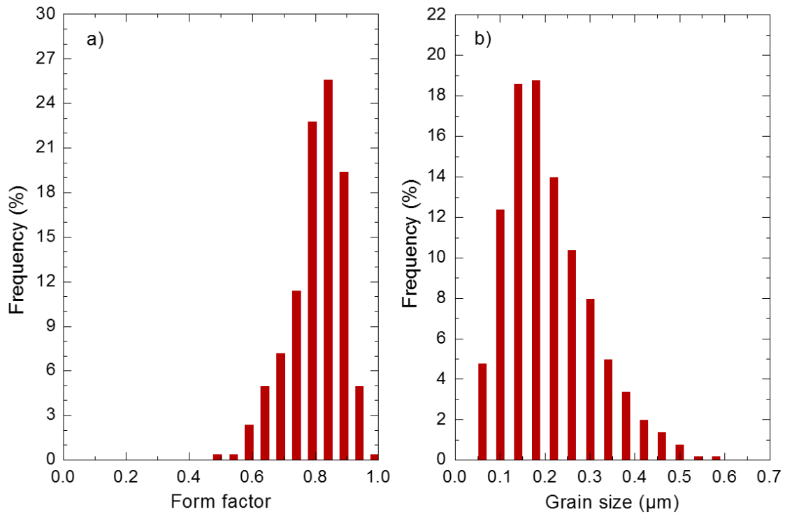
Fig. 3. Morphological distributions of BaZr 0.85 Y 0.15 O 2.925 : (a) Form factor; (b) Grain size.
