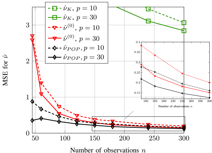
Fig. 1: Mean Square Errors of \hat{\nu} versus the number n of observations by running the different algorithms until convergence (MAX 5 iterations), using initial value \nu_0 . The samples are generated from a p -variate real t_3(\mathbf{0}, \Sigma) -distribution, where \Sigma has an AR(1) covariance matrix structure with \rho = 0.6 and p = 10 (dashed curves) and 30 (plain curves); 5000 Monte Carlo runs.
