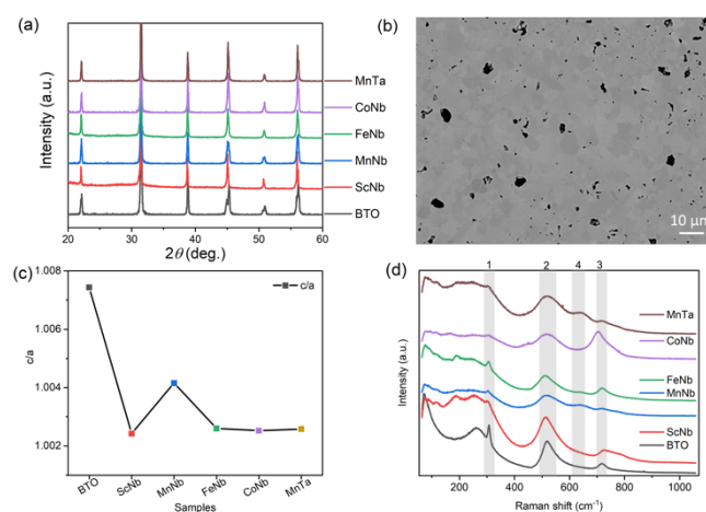
Fig. 1 (a) XRD patterns of the pure BTO and co-doped BTO samples measured at room temperature. (b) Typical microstructure of the ceramics (here the case of ( \text{Mn}^{3+} , \text{Nb}^{5+} ) co-doping). Black areas are pores and the different shades of grains come from different grain orientations as commonly observed in polycrystalline ceramics (c) Tetragonality i.e. c/a ratio depending on the dopants. (d) Raman spectra of undoped BTO and the co-doped samples collected at room temperature
