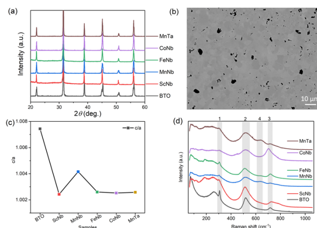
Fig. 1 (a) XRD patterns of the pure BTO and co-doped BTO samples measured at room temperature. (b) Typical microstructure of the ceramics (here the case of (\text{Mn}^{3+}, \text{Nb}^{5+}) co-doping). Black areas are pores and the different shades of grains come from different grain orientations as commonly observed in polycrystalline ceramics (c) Tetragonality i.e. c/a ratio depending on the dopants. (d) Raman spectra of undoped BTO and the co-doped samples collected at room temperature
