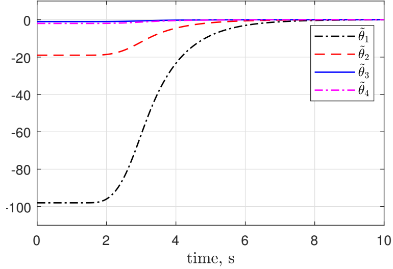
Figure 4: \tilde{\theta}(t) with DREM procedure and new LRE, estimator (35) and u_{pa}(t)
