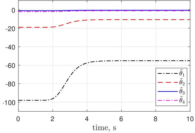
Figure 6: \tilde{\theta}(t) with DREM procedure, estimator (34) and u_{pb}(t)
