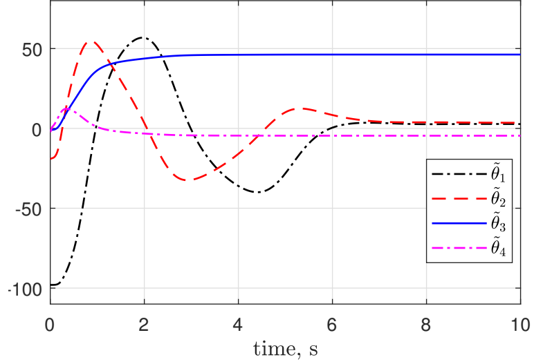
Figure 5: \tilde{\theta}(t) with gradient algorithm (33) and u_{pb}(t)
