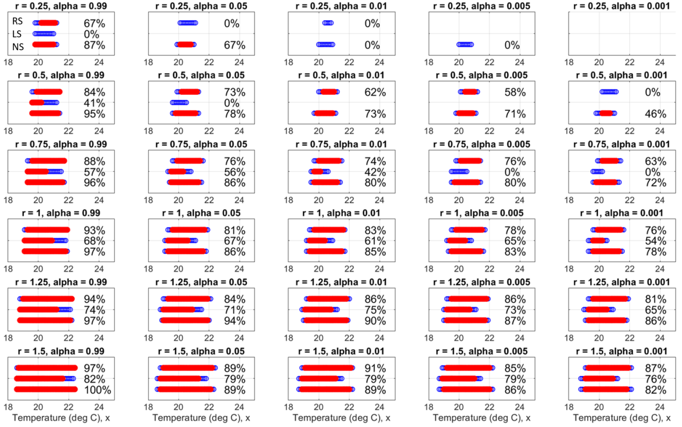
Fig. 4. For the temperature system with \gamma = 14 , estimates of the (\alpha, r, \gamma) -under-approximation set \mathcal{U}_{\alpha, \gamma}^r = \mathcal{U}_{\alpha, \gamma}^{r, \pi_\gamma} are shown (solid red circles). Estimates of the (\alpha, r) -risk-sensitive safe set for the control policy \pi_\gamma \in \Pi , \mathcal{S}_{\alpha, \gamma}^{r, \pi_\gamma} , are shown (white circles with blue boundary). Each plot presents the estimated sets for the different disturbance distributions (top interval: right skew (RS), middle interval: left skew (LS), and bottom interval: no skew (NS); see the labels in the first plot). Each percentage \frac{\text{Number of states in estimate of } \mathcal{U}_{\alpha, \gamma}^r}{\text{Number of states in estimate of } \mathcal{S}_{\alpha, \gamma}^{r, \pi_\gamma}} \cdot 100\% indicates the estimated quality of the under-approximation. These percentages are shown whenever the estimate of \mathcal{S}_{\alpha, \gamma}^{r, \pi_\gamma} is not empty. The risk-sensitivity level \alpha varies from nearly risk-neutral ( \alpha = 0.99 , left-most column) to more risk-averse ( \alpha = 0.001 , right-most column).
