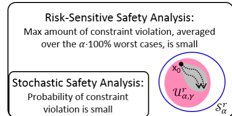
Fig. 2. We develop a safety analysis method that generalizes stochastic safety analysis by assessing the severity of random harmful outcomes. We define the risk-sensitive safe set \mathcal{S}_\alpha^r in terms of CVaR and derive an under-approximation \mathcal{U}_{\alpha, \gamma}^r that is computationally tractable. \mathcal{S}_\alpha^r represents the set of initial states from which the maximum extent of constraint violation of the state trajectory, averaged over the \alpha \cdot 100\% worst cases, can be reduced to a threshold r .
