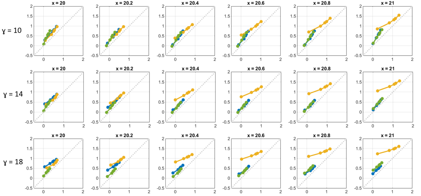
Fig. 3. Computations of the inequality that we have proved in Theorem 1 are shown for the temperature system. In each plot, the horizontal axis provides estimates of \text{CVaR}_{\alpha,x}^{\pi,\gamma}(\max_{t=0,1,\dots,T} g_K(X_t)) , and the vertical axis provides estimates of \frac{1}{\gamma} \log\left(\frac{1}{\alpha} E_x^{\pi,\gamma}\left(\sum_{t=0}^T e^{\gamma g_K(X_t)}\right)\right) for 5 different risk-sensitivity levels \alpha \in \Lambda := \{0.99, 0.05, 0.01, 0.005, 0.001\} . Points associated with smaller values of \alpha (more risk-averse) are positioned farther away from the origin. For a fixed \gamma , \pi_\gamma is an optimal (deterministic, Markov) policy for the MDP problem (23). In each plot, there are three solid colored lines, one for each distribution of the disturbance process (green = no skew, yellow = left skew, blue = right skew). In each plot, \gamma \in \{10, 14, 18\} and an initial state x \in \{20, 20.2, \dots, 21\} are fixed. The value of \gamma varies along the rows, and the value of x varies along the columns. A dotted gray line of slope 1 is shown for visual comparison.
