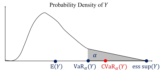
Fig. 1. The Conditional Value-at-Risk (CVaR) quantifies the upper tail of a cost distribution. For an absolutely continuous, bounded random variable Y representing a cost and \alpha \in (0, 1] , we illustrate the expected cost in the \alpha \cdot 100\% worst cases, which is CVaR_\alpha(Y) in this setting. The area of the shaded region is \alpha . The expectation of Y , the Value-at-Risk of Y at level \alpha (the lowest cost in the \alpha \cdot 100\% worst cases), and the essential supremum of Y are also shown.
