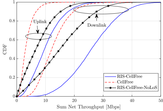
Fig. 4. CDF of the sum net throughput [Mbps] with M = 100 , K = 10 , N = 900 , \tau_p = 5 , and d_H = d_V = \lambda/4 . The unblocked probability of the direct links is \bar{p} = 0.2 .
