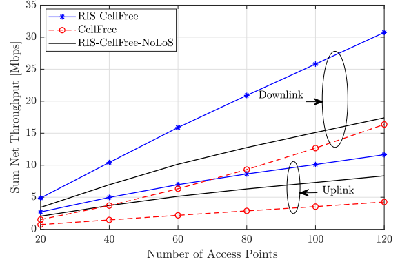
Fig. 5. Average sum net throughput [Mbps] versus the number of APs with K = 10 , N = 900 , \tau_p = 5 , and d_H = d_V = \lambda/4 . The unblocked probability of the direct links is \bar{p} = 0.2 .
