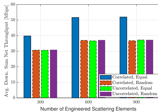
Fig. 9. Average downlink sum net throughput [Mbps] versus the number of engineered scattering elements with M = 100 , K = 10 , \tau_p = 5 , and d_H = d_V = \lambda/4 . The unblocked probability of the direct links is \bar{p} = 0.2 .
