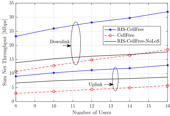
Fig. 6. Average sum net throughput [Mbps] versus the number of users with M = 100 , N = 900 , \tau_p = 5 , and d_H = d_V = \lambda/4 . The unblocked probability of the direct links is \bar{p} = 0.2 .
