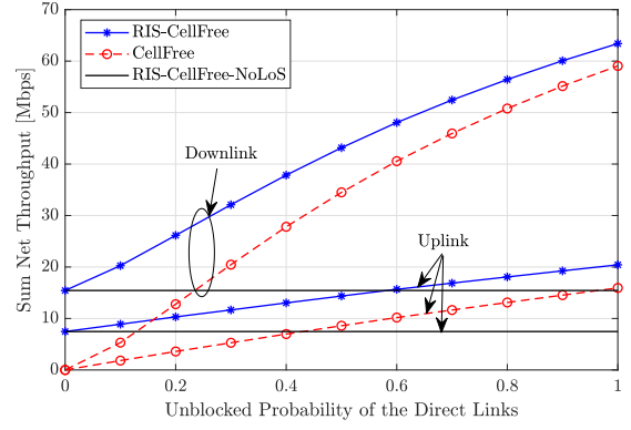
Fig. 3. Average sum net throughput [Mbps] versus the unblocked probability of the direct links \bar{p} with M = 100 , K = 10 , N = 900 , \tau_p = 5 , and d_H = d_V = \lambda/4 .
