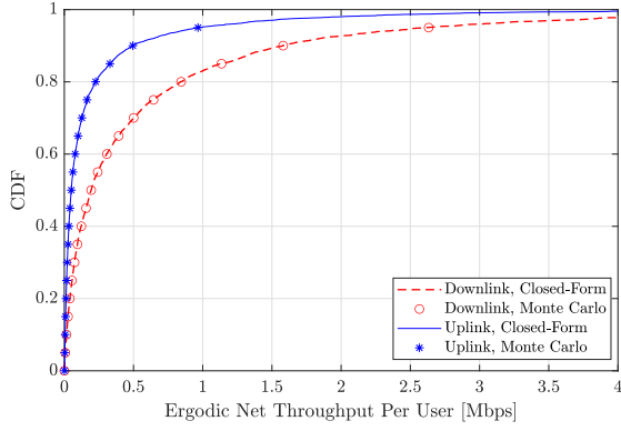
Fig. 2. Monte Carlo simulations versus the analytical frameworks with M = 20 , K = 5 , N = 64 , \tau_p = 2 , and d_H = d_V = \lambda/4 . The unblocked probability of the direct links is \bar{p} = 1.0 .
