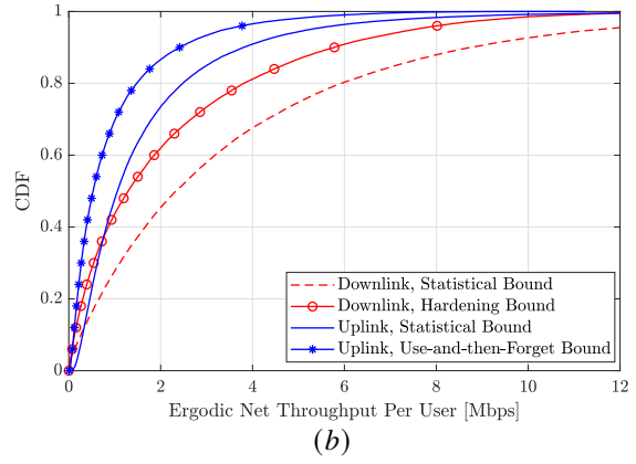
Fig. 12. A comparison of different channel capacity bounding techniques with M = 20 , K = 10 , N = 64 , \tau_P = 10 , d_H = d_V = \lambda/4 , \tilde{p} = 1.0 , and two coherence intervals: (a) \tau_c = 200 symbols; (b) \tau_c = 5000 symbols.
