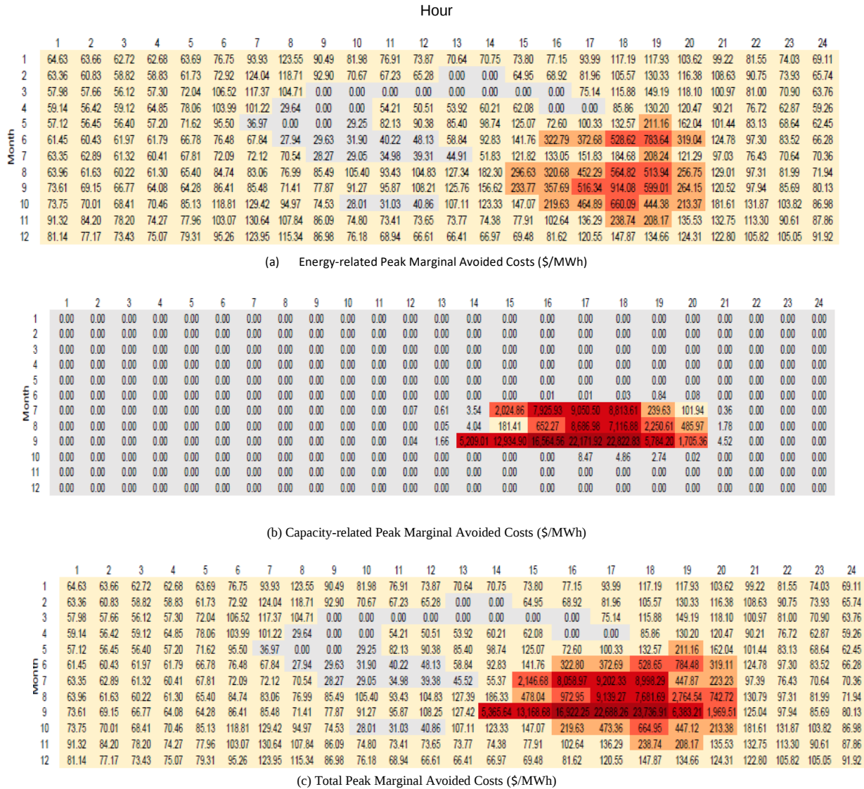
Figure 2: Marginal peak avoided costs profile for Forecasting Climate Zone 9 in 2020
