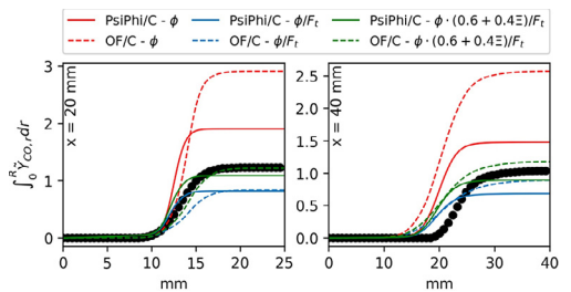
Fig. 10. Integration of the mean mass fraction of CO at several location above the burner on the radial direction for coarse simulations. Red lines: uncorrected \langle \hat{Y}_{CO} \rangle . Blue lines: with laminar correction \langle \hat{Y}_{CO}^c \rangle . Green lines: with turbulent correction \langle \hat{Y}_{CO}^{c,T} \rangle . Dashed lines: OpenFOAM. Solid lines: PsiPhi (coarse grid). (For interpretation of the references to color in this figure legend, the reader is referred to the web version of this article.)
