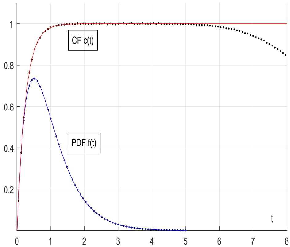
Fig. 2. Erlang (2) Process : PDF and CF. Continuous curves : Theory ; Points : experiments.
