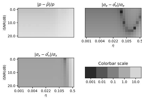
Fig. 4. Recovery of the parameters on blurry simulated signals.
