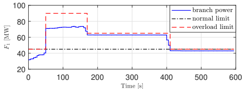
Fig. 5. Power flow of line 1 in Scenario 2.
