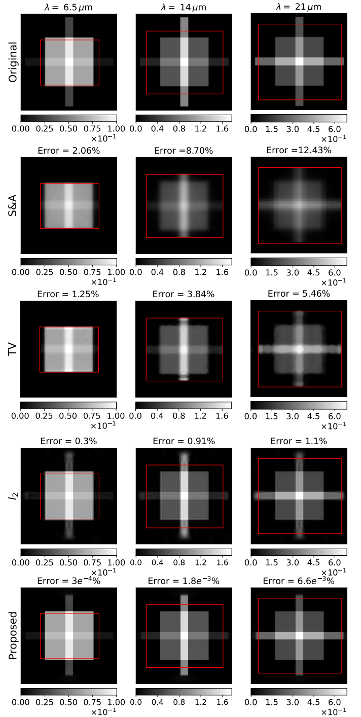
Fig. 9. Spatial reconstruction for Obj_1 : Original images at 6.5, 14, and 21\mu m [1st row], S&A [2nd row], TV restoration [3rd row], l_2 approach [4th row], proposed [5th row].
