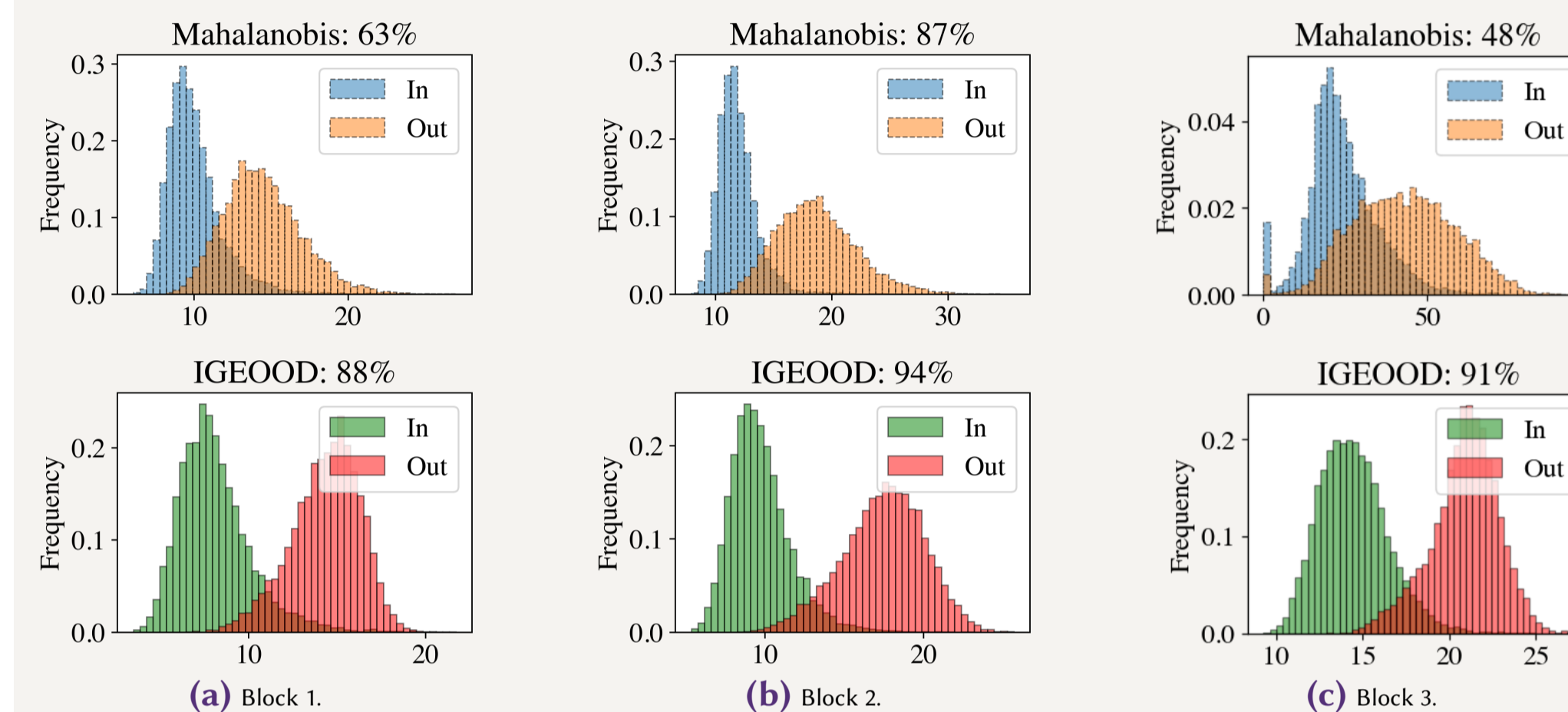
Figure: Histograms of the Mahalanobis and IGEOD scores for the outputs of each hidden block of a DenseNet model on CIFAR-10 (in-distribution) and SVHN (out-of-distribution) datasets.
