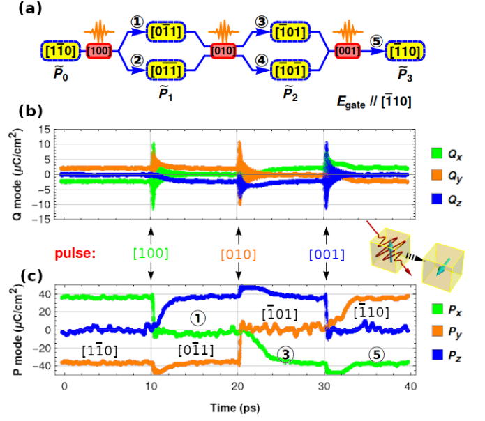
FIG. 3. Deterministic full-reversal strategy: (a) protocol of the three-pulse reversal process; the yellow background boxes are for the initial and excited polarization phases and the pink background boxes are used to indicate the laser pulses that are along x, y, and z-axis; The labels of the phases \tilde{\mathbf{P}} is defined as \mathbf{P} + \mathbf{Q} to indicate the total polarization; The blue arrows are used to indicate the phase transition channels after the laser pulses; Responses of the \mathbf{Q} (b) and \mathbf{P} modes (c) excited by a sequence of three “200fs-18THz” pulses activated at 10, 20, and 30 ps and having their polarized direction along [100] , [010] , and [011] directions, respectively. For each of these pulses, the magnitude of \mathbf{E} in \mathbf{E}e^{-2\ln 2(\frac{t}{\tau})^2} \cos(2\pi\omega t) is 6.17 MV/cm.
