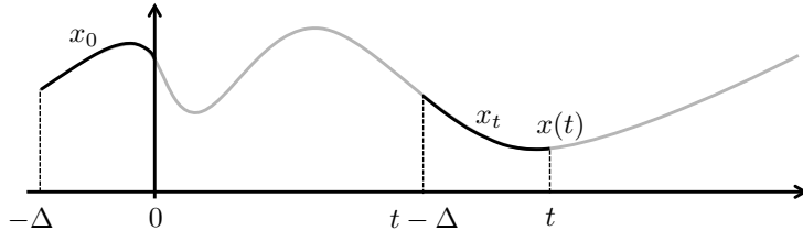
Figure 1: Time evolution of the solution of (1).
