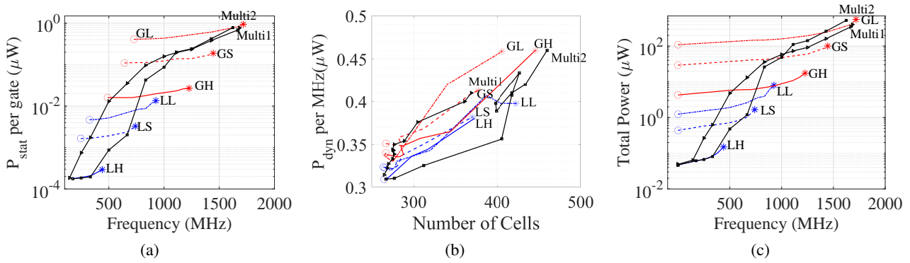
Figure 4: Analysis of static and dynamic power consumption as a function of the synthesis constraints: (a) P_{stat} per gate over clock frequency, (b) P_{dyn} per MHz over the number of gates, and (c) total power consumption over clock frequency.
