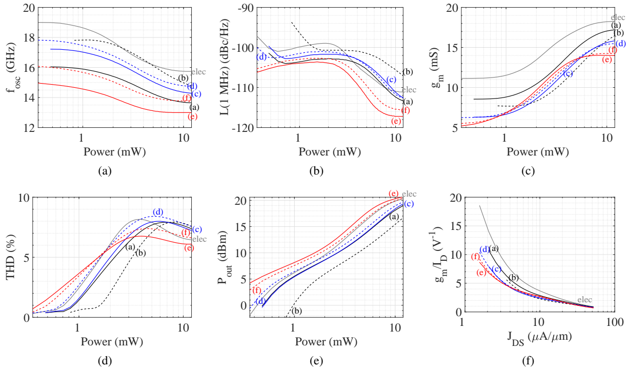
Figure 15: Voltage controlled oscillator post-layout simulation results over power consumption compromise: (a) speed from f_{osc} , (b) noise from L(1\text{ MHz}) , (c) gain from g_m , (d) linearity from THD, (e) dynamic range from P_{out} , analysis and (f) g_m/I_D characteristics over layout parasitic.
