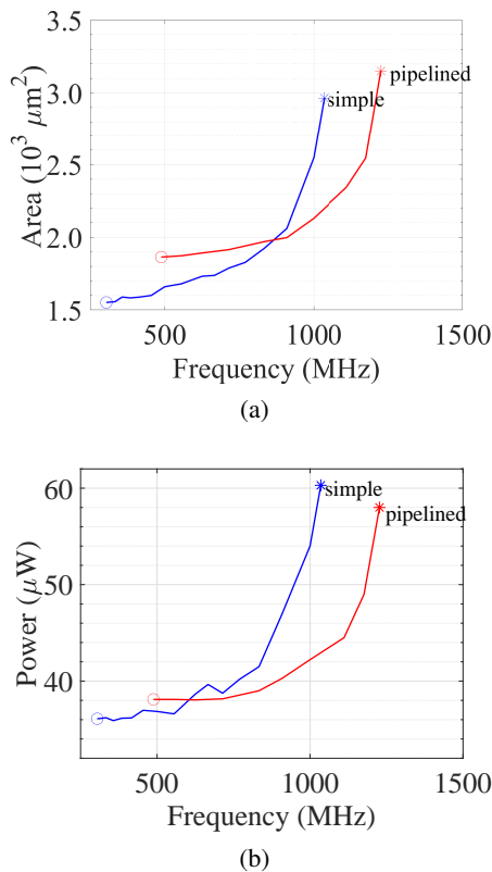
Figure 2: Compromises in 16-bit synchronous gray counter followed by a gray-to-binary synchronous decoder synthesis, being (a) maximum frequency and area, and (b) maximum frequency and power consumption.
