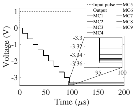
Figure 10: Time domain Monte Carlo Analysis for Input signal (dotted line) and nine-sample output signal (continuous line)
