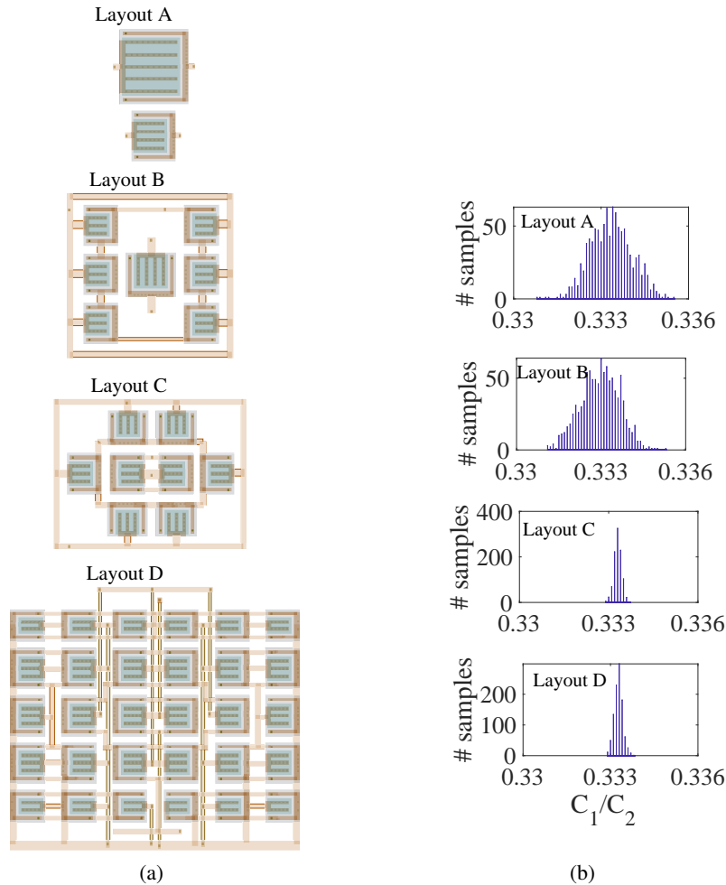
Figure 11 (a) C_1/C_2 Capacitor Layout, and (b) histogram for 1000-point Monte Carlo PLS results for Case A, B, C and D.
