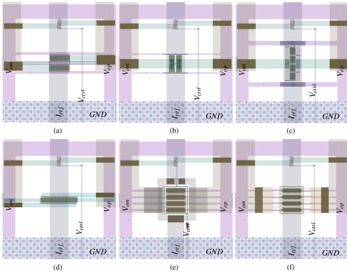
Figure 14: Voltage controlled oscillator layout ( 59 \times 63 \mu\text{m}^2 ): (a) classic using automatic routing and Pcell constraints, (b) classic using manual routing and custom cells, (c) full custom considering common-centroid interdigitated cells in four lines, (d) full custom considering common-centroid interdigitated cells in one line, (e) full-custom RF technique considering double-gate access, EM propagation common centroid interdigitated cells for thicker Metal8 routing, and (f) full-custom RF technique for a thinner Metal5 routing.
