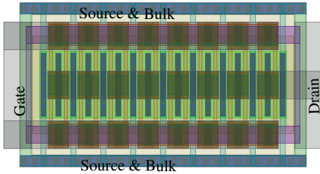
Figure 12: Transistor layout topology considering a minimum of extrinsic RF parasitic elements added in intrinsic transistor core
