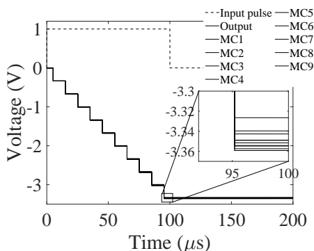
Figure 10: Time domain Monte Carlo Analysis for Input signal (dotted line) and nine-sample output signal (continuous line)
