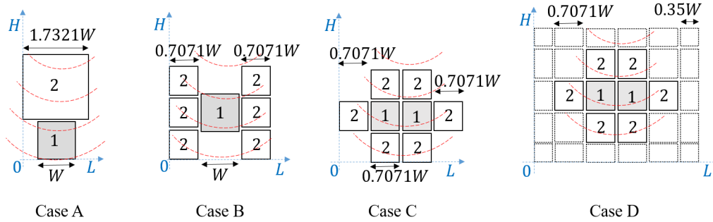
Figure 7 Considered topologies for capacitance ratio layout. Red dotted lines represent gradient lines.
