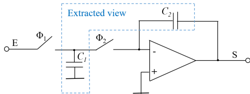
Figure 9: Test bench illustration for a switched capacitor integrator under test.
