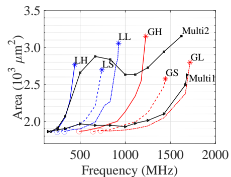
Figure 3: Compromises in the proposed digital function synthesis in terms of maximum frequency and area for LL, GL, LS, GS, LH, and GH single gate library families; for Multi1 (no power constraint) and Multi2 (minimal leakage current).
