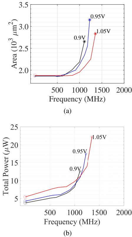
Figure 5: GH library compromises over V_{DD} selection, being (a) maximum frequency and area, and (b) maximum frequency and power consumption.
