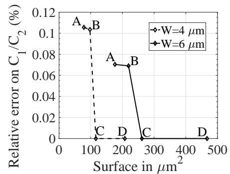
Figure 8 Relative error on C_1/C_2 as a function of surface.
