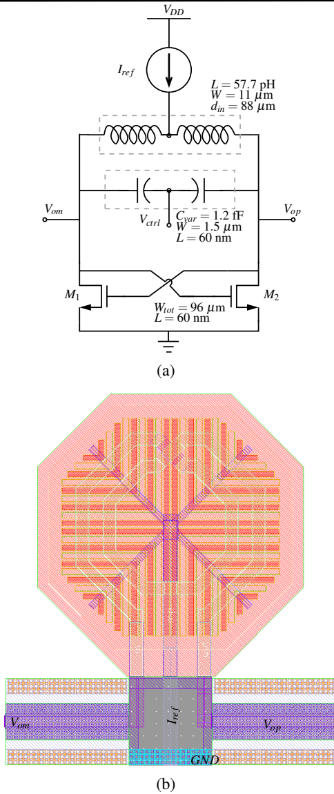
Figure 13: Voltage controlled oscillator under test: (a) the schematic, and (b) the layout ( 241 \times 270 \mu\text{m}^2 ) illustration.
