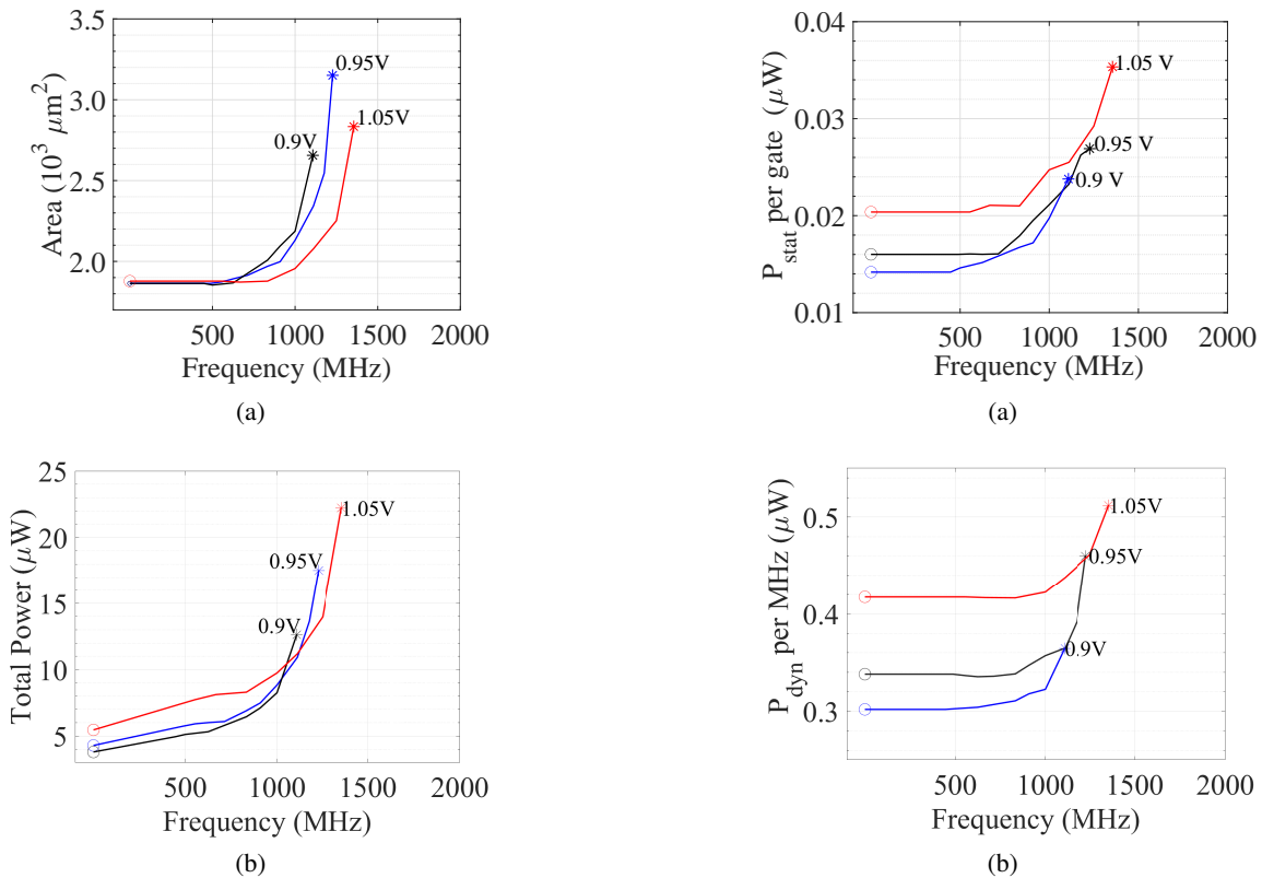
Figure 5: GH library compromises over V_{DD} selection, being (a) maximum frequency and area, and (b) maximum frequency and power consumption.
