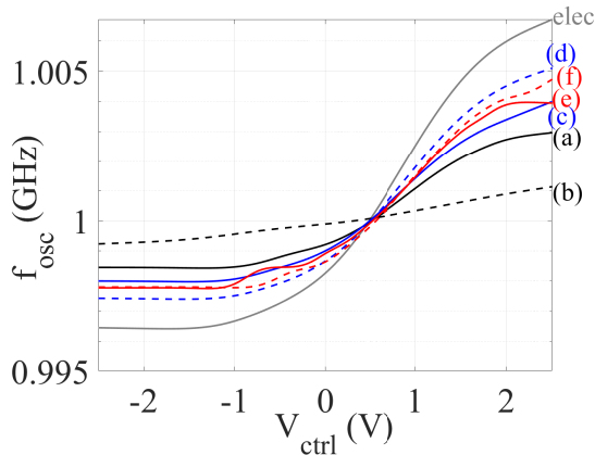
Figure 16: VCO speed performance ( f_{osc} ) reconfiguration over control voltage ( V_{ctrl} ) normalized to the average one for each layout case (see Tab. II).
