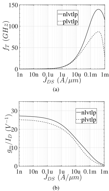
Figure 1: B55 characteristics extraction for low-threshold voltage low-power NMOS (nlvtlp) and PMOS (plvtlp) transistors, being (a) the f_T and (b) the g_m/I_D versus J_{DS} .
