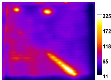
Fig. 1 : EL image of 1cm 2 monocrystalline Si-IBC at 0.9V bias applied. We note locally reduced EL emission due to variation of electronic properties.
