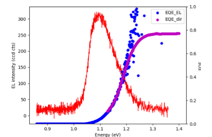
Fig. 3 : Comparison of EL spectra (red curves) and quantum efficiencies (magenta point). The blue points represent the quantum efficiencies that follow from the EL spectra.
