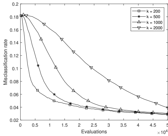
Figure 10: Average performance metrics volume of the symmetric difference (top) and misclassification rate (bottom) for problem g_5 , when considering k of 200, 500, 1000 and 2000.
