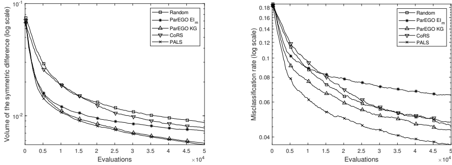
Figure 11: Average volume of the symmetric difference (left) and misclassification rate (right) on test problem g_8 for PRS, CoRS, ParEGO- El_m , ParEGO-KG and PALS.
