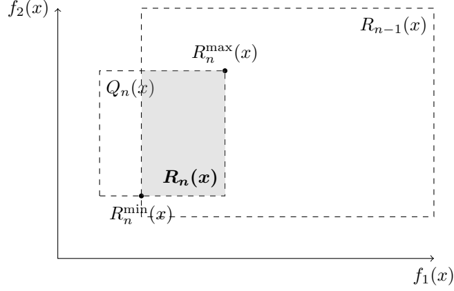
Figure 4: Bi-objective example of the construction of a classification region R_n(x) (filled region), and the respective optimistic R_n^{\max}(x) and pessimistic R_n^{\min}(x) outcomes.
