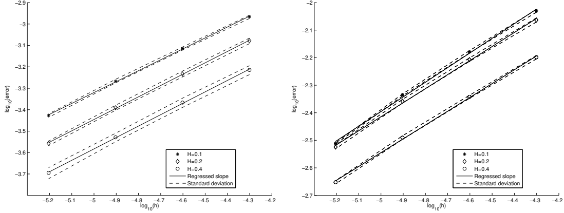
Figure 1: Plot of the logarithm of the strong error ( y -axis) against h ( x -axis) for a bounded drift. Left: Equation (6.8) ( d = 1 ) - Right: Equation (6.7) ( d = 2 ). For different values of H < 1/2 , and in both dimension 1 and 2, we observe that the numerical order of convergence (by linear regression) is approximately 0.5 (with a standard deviation plotted in dashed lines), which coincides with the theoretical order 1/2 .
