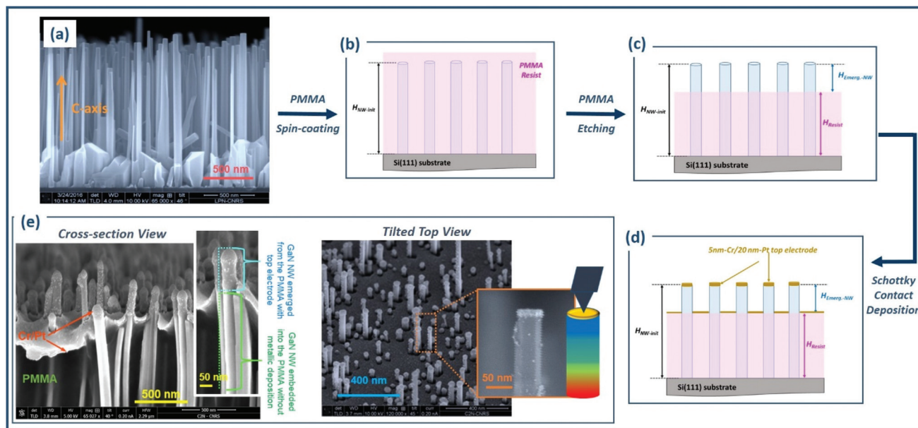
Fig. 2 (a) GaN NWs grown by plasma-assisted molecular beam epitaxy; (b–d) schematic representation of the preparation for the GaN NW sample for AFM measurements. H_{NW-init} , H_{Embed-NW} and H_{resist} define respectively the initial NW height, the protruding NW height after consolidation and the resist height; (e) SEM images of tilted top view and cross-section view of the electrically connected NWs with a thin 5 nm-Cr/20 nm-Pt Schottky electrode directly deposited on the top of each NW forming the array.
