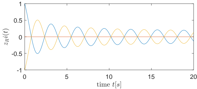
Fig. 5. Simulations results of N_R = 3 reduced order system
