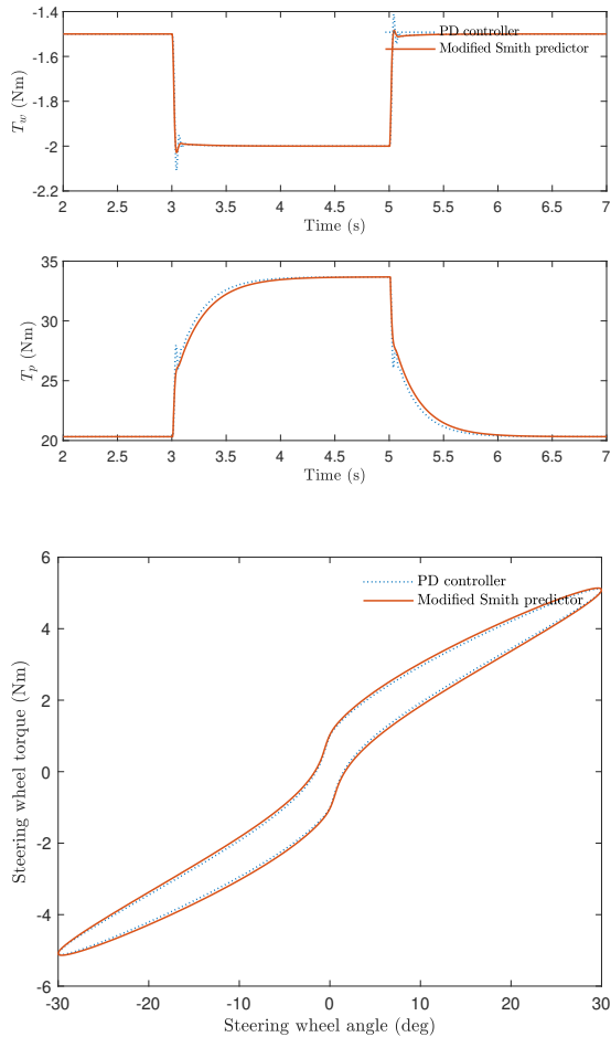
Fig. 11: Case 2: (top) Control signals for a square-like steering torque input. (bottom) SBW steering feel for a sinusoidal driver torque input.
