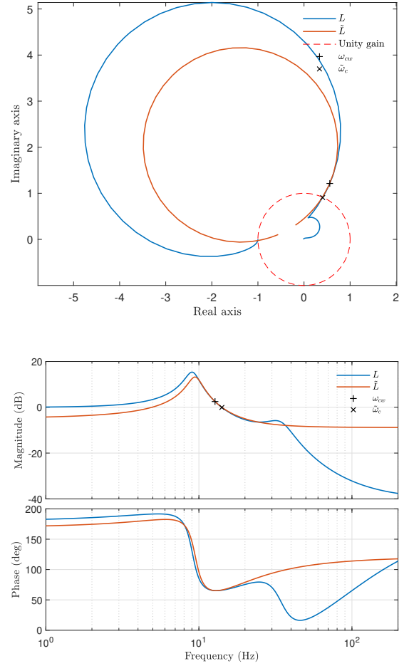
Fig. 6: Approximation at \omega_{cw} of the open-loop transfer function L , for \tau_w = \tau_p = 5 ms: (top) Nyquist locus. (bottom) Bode diagram.
