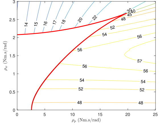
Fig. 8: Delay margin contours, in (ms), for \tau_w = \tau_p = 5 ms. The conditions of Proposition 2 do not hold inside the domain bounded by the red curve.
