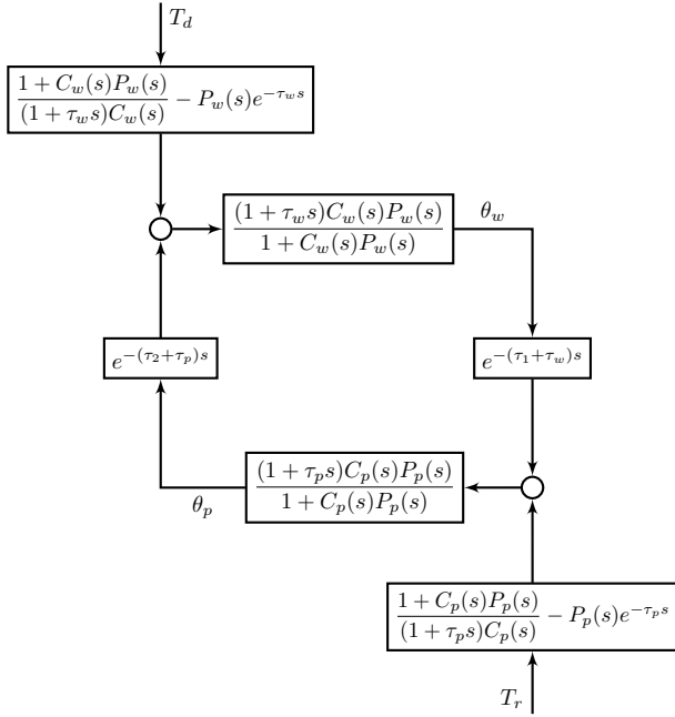
Fig. 5: SBW block diagram with modified Smith predictor controllers.
