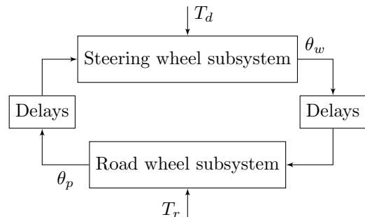
Fig. 1: SBW block diagram.
