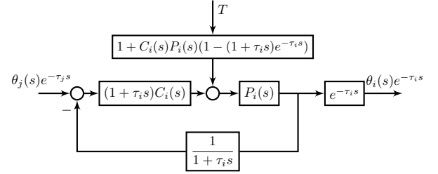
Fig. 4: Steering wheel/Road wheel subsystems block diagram with modified Smith predictor.
