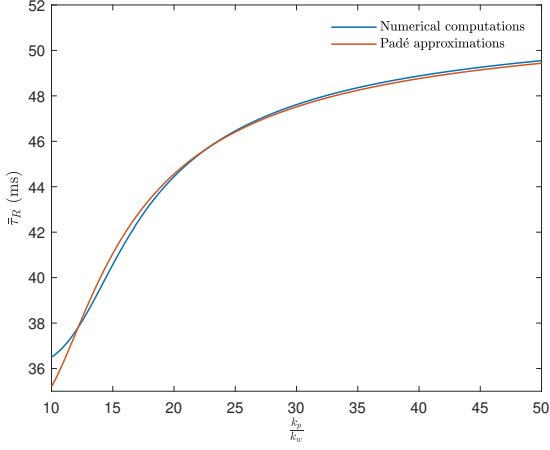
Fig. 7: Comparison between the delay margins \bar{\tau}_R at several values of \frac{k_p}{k_w} , for \tau_w = \tau_p = 5 ms.
