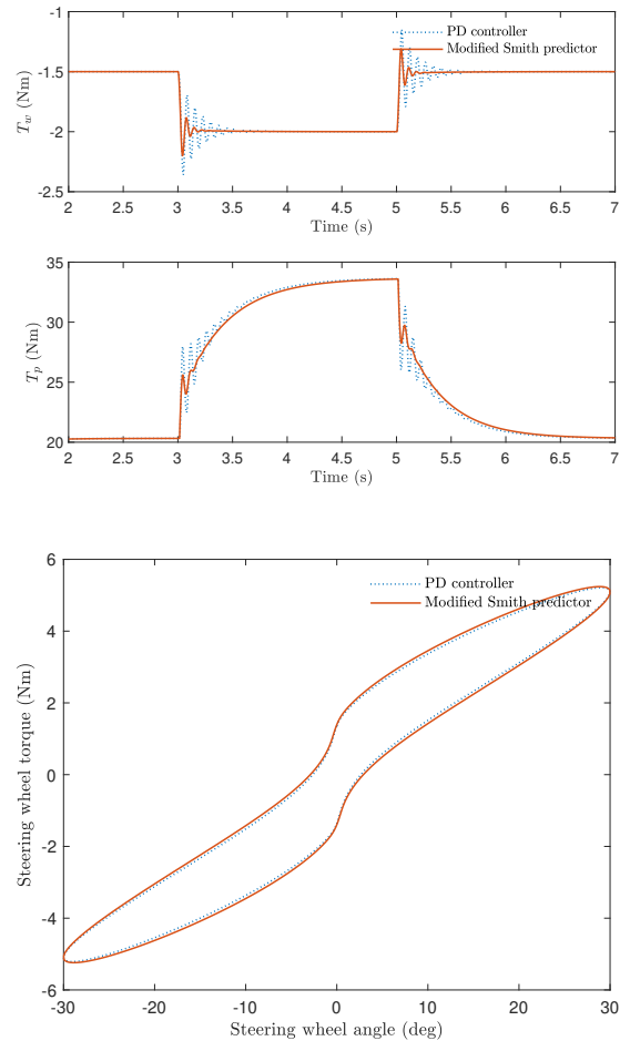
Fig. 12: Case 3: (top) Control signals for a square-like steering torque input. (bottom) SBW steering feel for a sinusoidal driver torque input.
