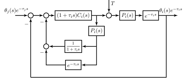
Fig. 3: Steering wheel/Road wheel subsystems block diagram with modified Smith predictor.
