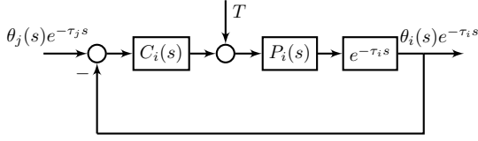
Fig. 2: Steering wheel/Road wheel subsystems block diagram with PD controller.
