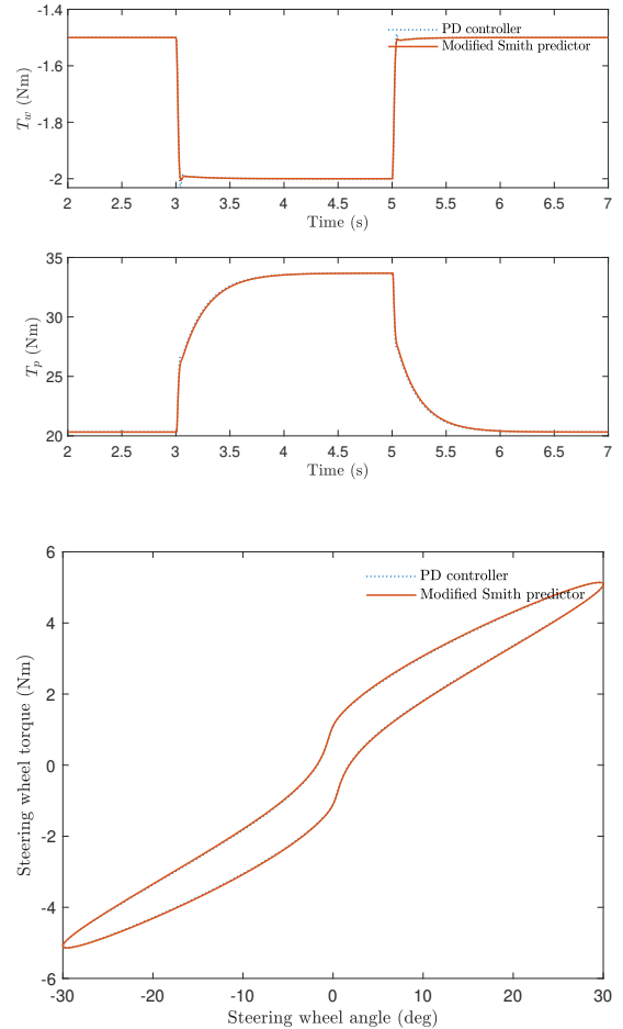
Fig. 10: Case 1: (top) Control signals for a square-like steering torque input. (bottom) SBW steering feel for a sinusoidal driver torque input.
