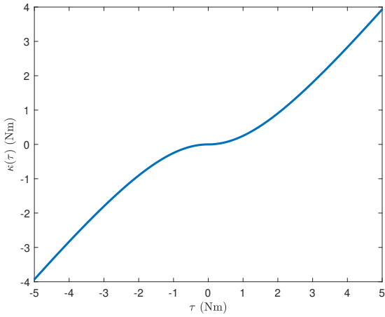
Fig. 9: Normalized nonlinear torque map.
