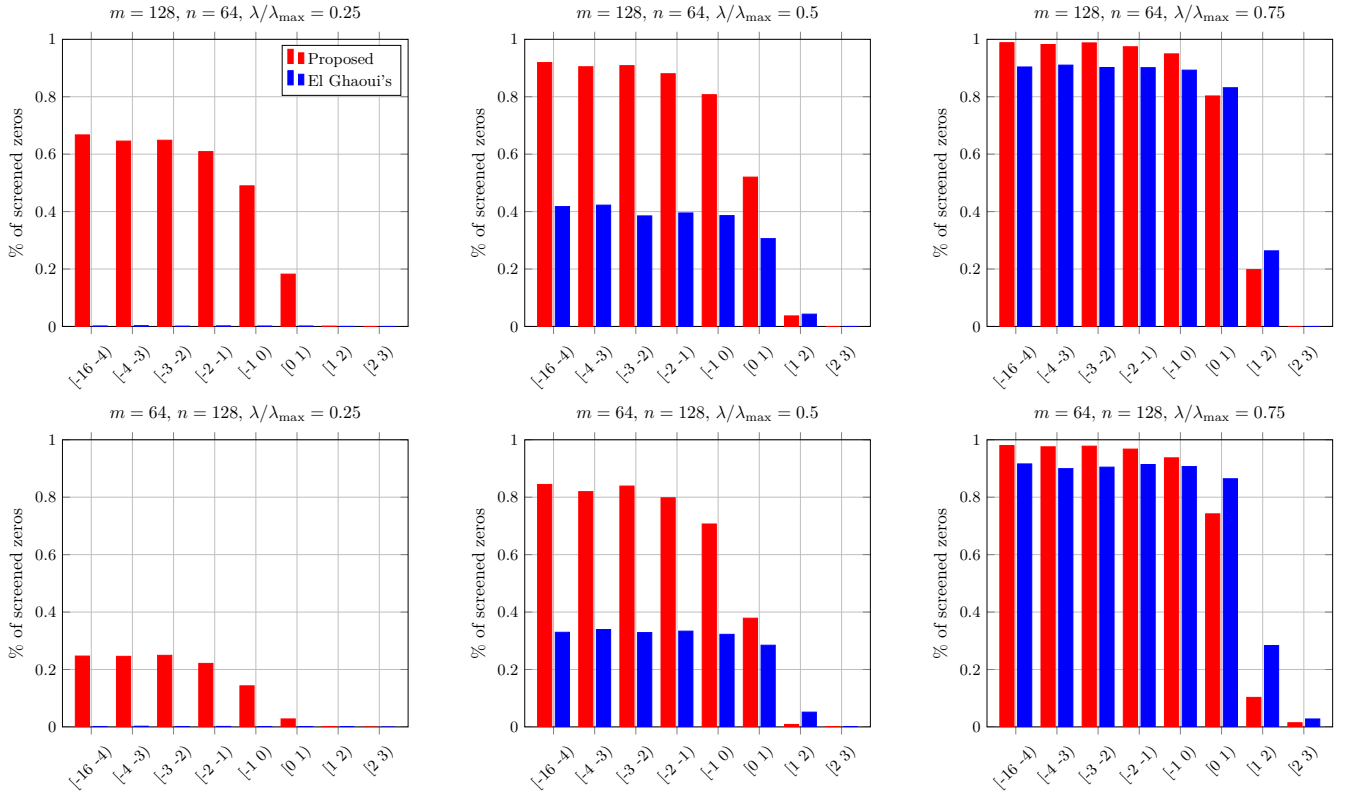
Figure 1. Percentage of zeros in the minimizers of (26) identified by the screening tests as a function of the duality gap attained by the couple (\bar{\mathbf{x}}, \bar{x}, \bar{\mathbf{u}}) used in the tests. The results are averaged over 100 problem instances. Blue: El Ghaoui et al. 's test [7]; Red: our region-free test (17).
