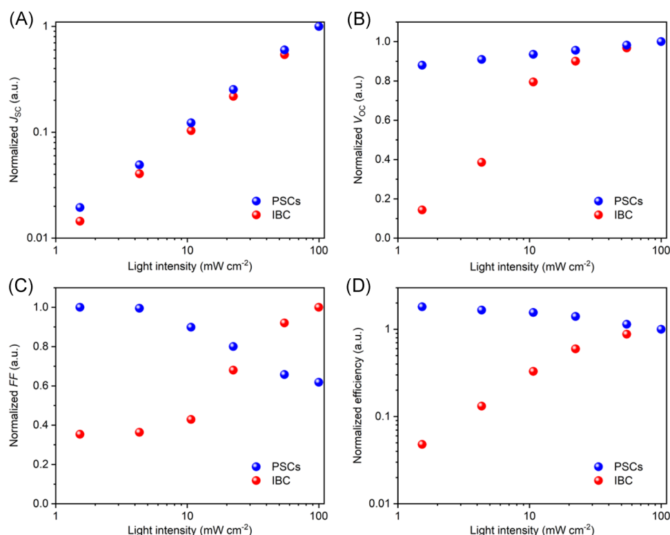
FIGURE 3 Photovoltaic performances as a function of light intensity of (A) J SC , (B) V OC , (C) FF , and (D) photoconversion efficiency for PSC top and interdigitated back contact (IBC) bottom cells. Each plot is normalized to the highest value
