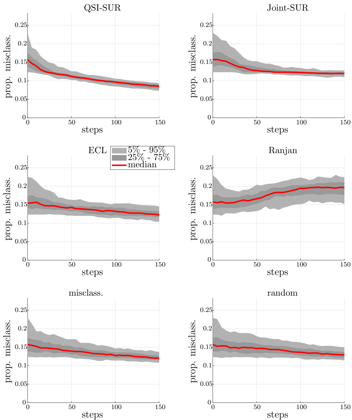
Figure SM6: Median and several quantiles of the proportion of misclassified points vs. number of iterations, for 100 repetitions of the algorithms on the test function f_2 .
