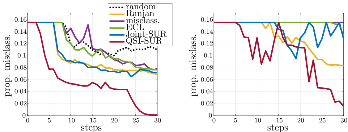
Figure 4: Quantiles of order 0.75 (left) and 0.95 (right) of the proportion of misclassified points vs. number of iterations, for 100 repetitions of the algorithms on the test function f_1 .
