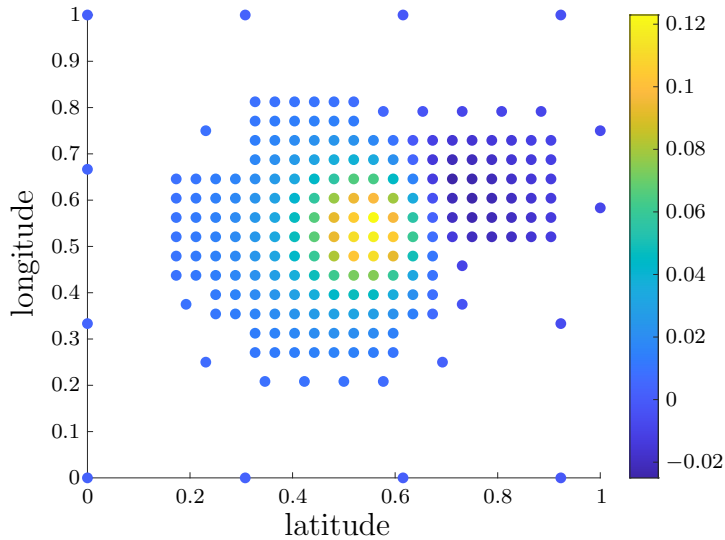
Figure 6: True measures of the displacement at the volcano surface with respect to the normalized latitude and longitude.
