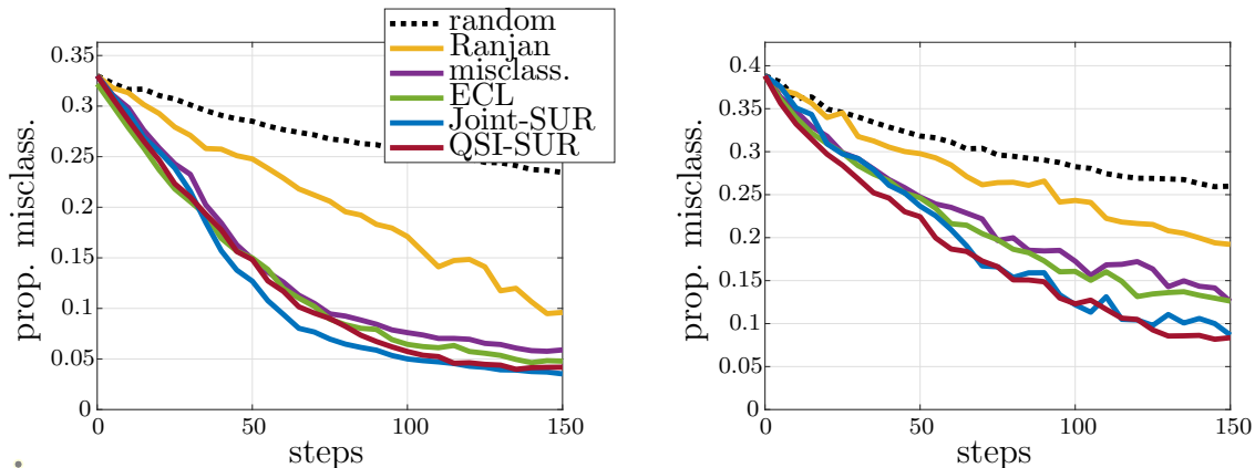
Figure 7: Median (left) and quantile of order 0.95 (right) of the proportion of misclassified points vs. number of iterations, for 100 repetitions of the algorithms on “volcano” test case.
