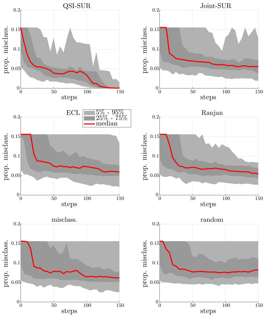
Figure SM3: Median and several quantiles of the proportion of misclassified points vs. number of iterations, for 100 repetitions of the algorithms on the test function f_1 .
