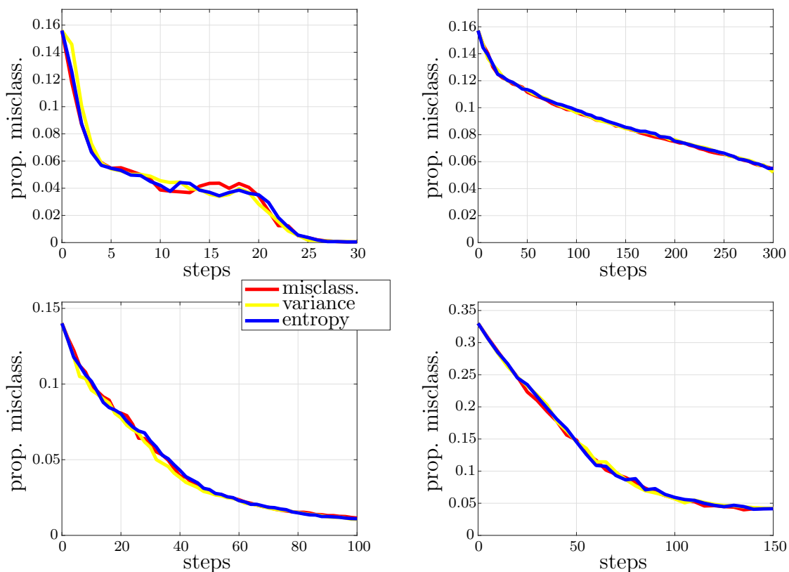
Figure SM1: Median of the proportion of misclassified points vs. number of iterations, for 100 repetitions of the algorithms on the test functions f_1 (top left), f_2 (top right), f_3 (bottom left) and the volcano case (bottom right).
