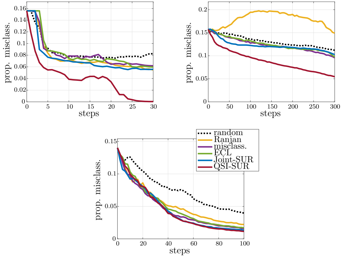
Figure 3: Median of the proportion of misclassified points vs. number of iterations, for 100 repetitions of the algorithms on the test functions f_1 (top left), f_2 (top right) and f_3 (bottom).
