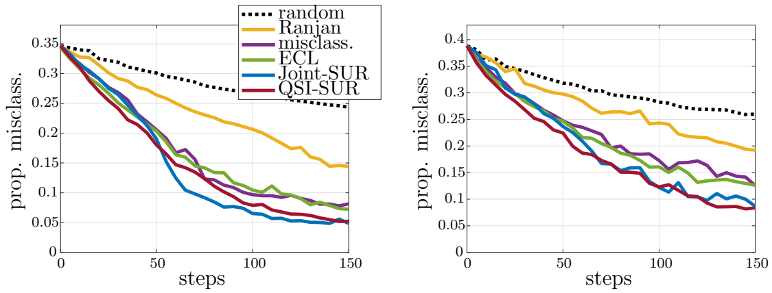
Figure SM11: Quantiles of level 0.75 and 0.95 for the proportion of misclassified points vs. number of iterations, for 100 repetitions of the algorithms on the test case volcano.
