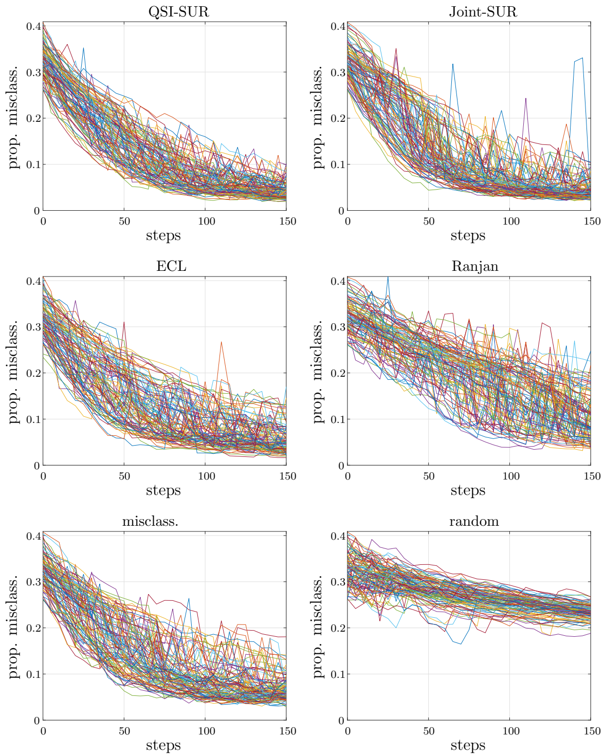
Figure SM13: Different sample paths of the proportion of misclassified points vs. number of iterations, for 100 repetitions of the algorithms on the test case volcano.
