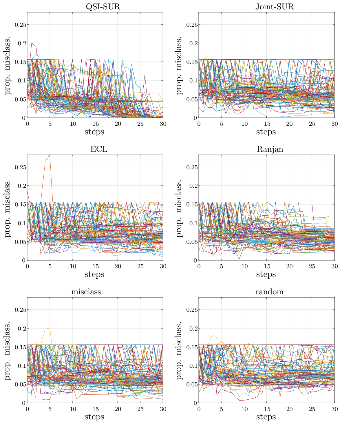
Figure SM4: Different sample paths of the proportion of misclassified points vs. number of iterations, for 100 repetitions of the algorithms on the test function f_1 .
