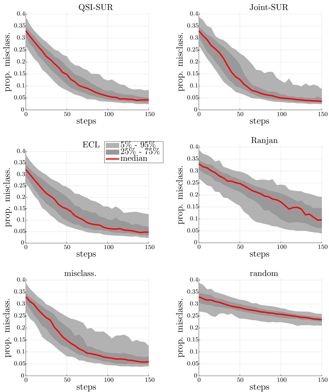
Figure SM12: Median and several quantiles of the proportion of misclassified points vs. number of iterations, for 100 repetitions of the algorithms on the test case volcano.
