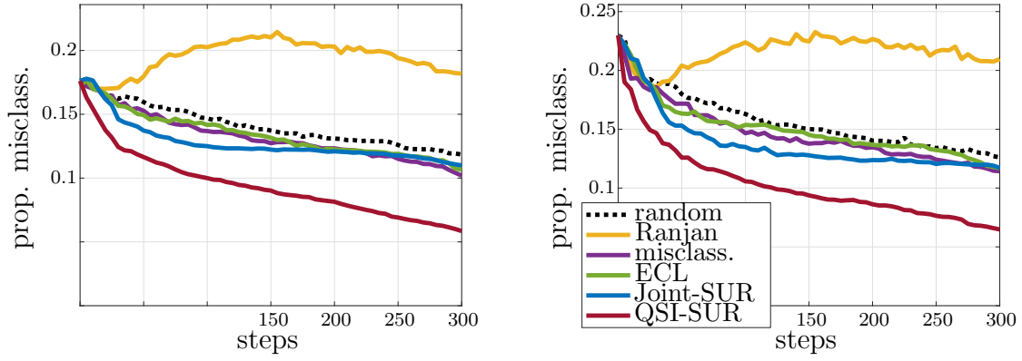
Figure SM5: Quantiles of level 0.75 and 0.95 for the proportion of misclassified points vs. number of iterations, for 100 repetitions of the algorithms on the test function f_2 .
