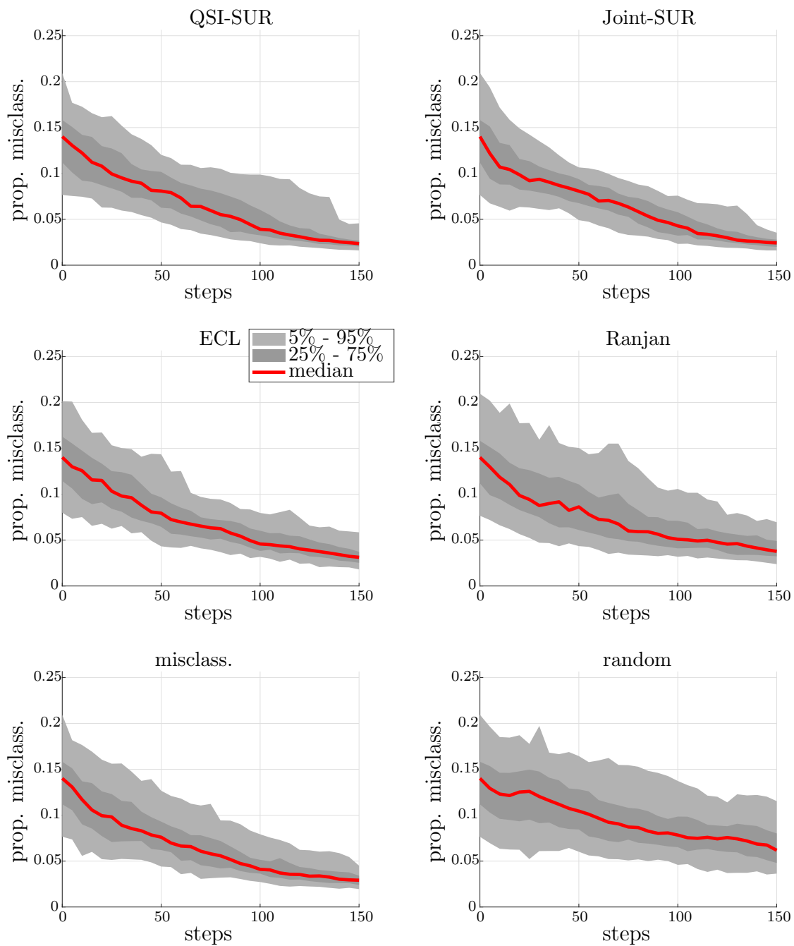
Figure SM9: Median and several quantiles of the proportion of misclassified points vs. number of iterations, for 100 repetitions of the algorithms on the test function f_3 .
