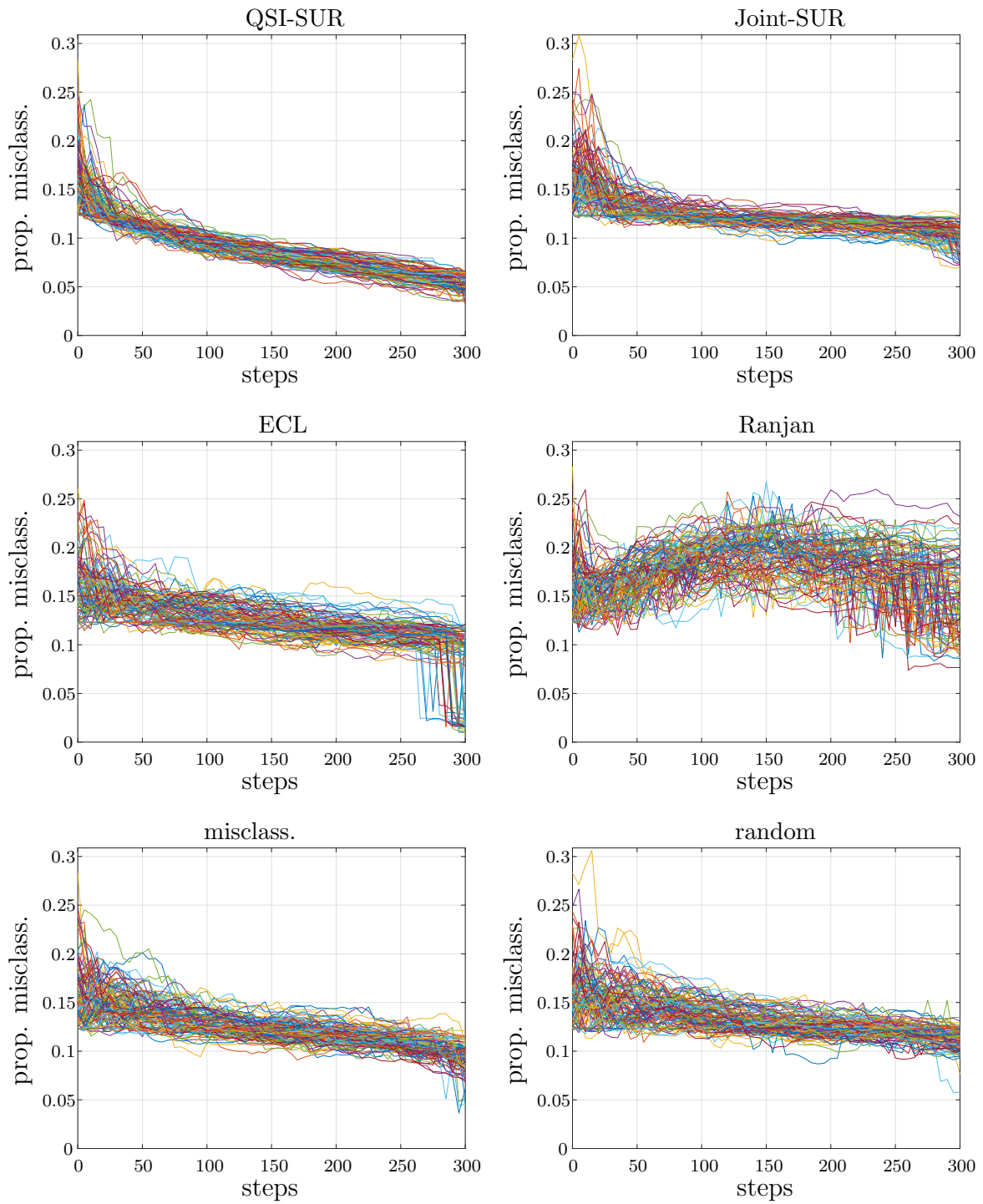
Figure SM7: Different sample paths of the proportion of misclassified points vs. number of iterations, for 100 repetitions of the algorithms on the test function f_2 .
