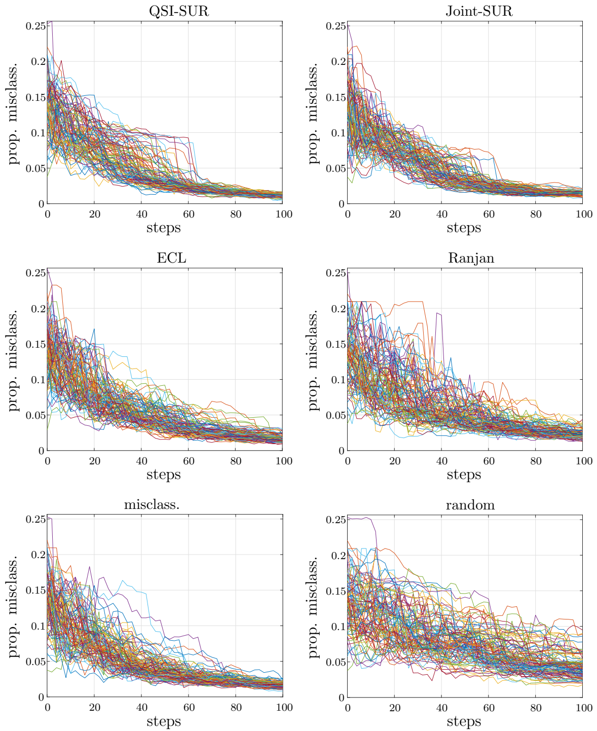
Figure SM10: Different sample paths of the proportion of misclassified points vs. number of iterations, for 100 repetitions of the algorithms on the test function f_3 .
